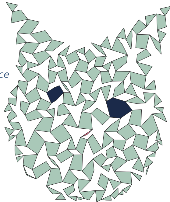
deployed, \theta = 0.70
