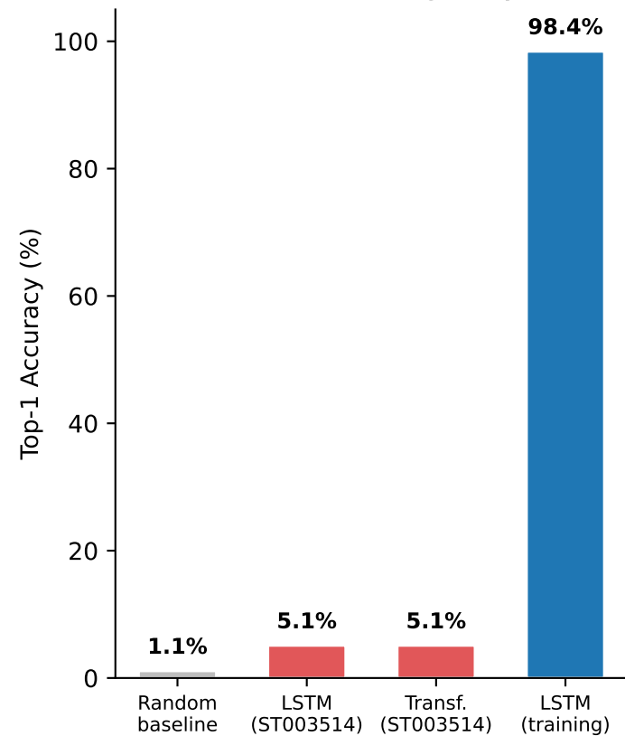
(C) Different chromatography
