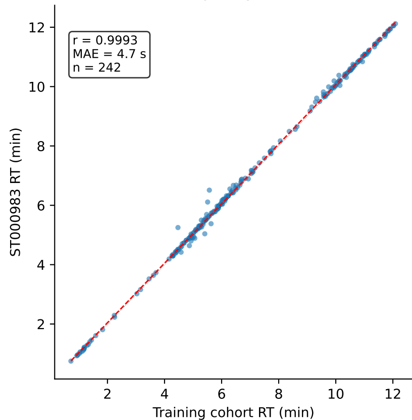
(A) Same chromatography, different MS
