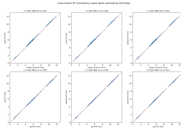
(B) Within-training cross-cohort RT
