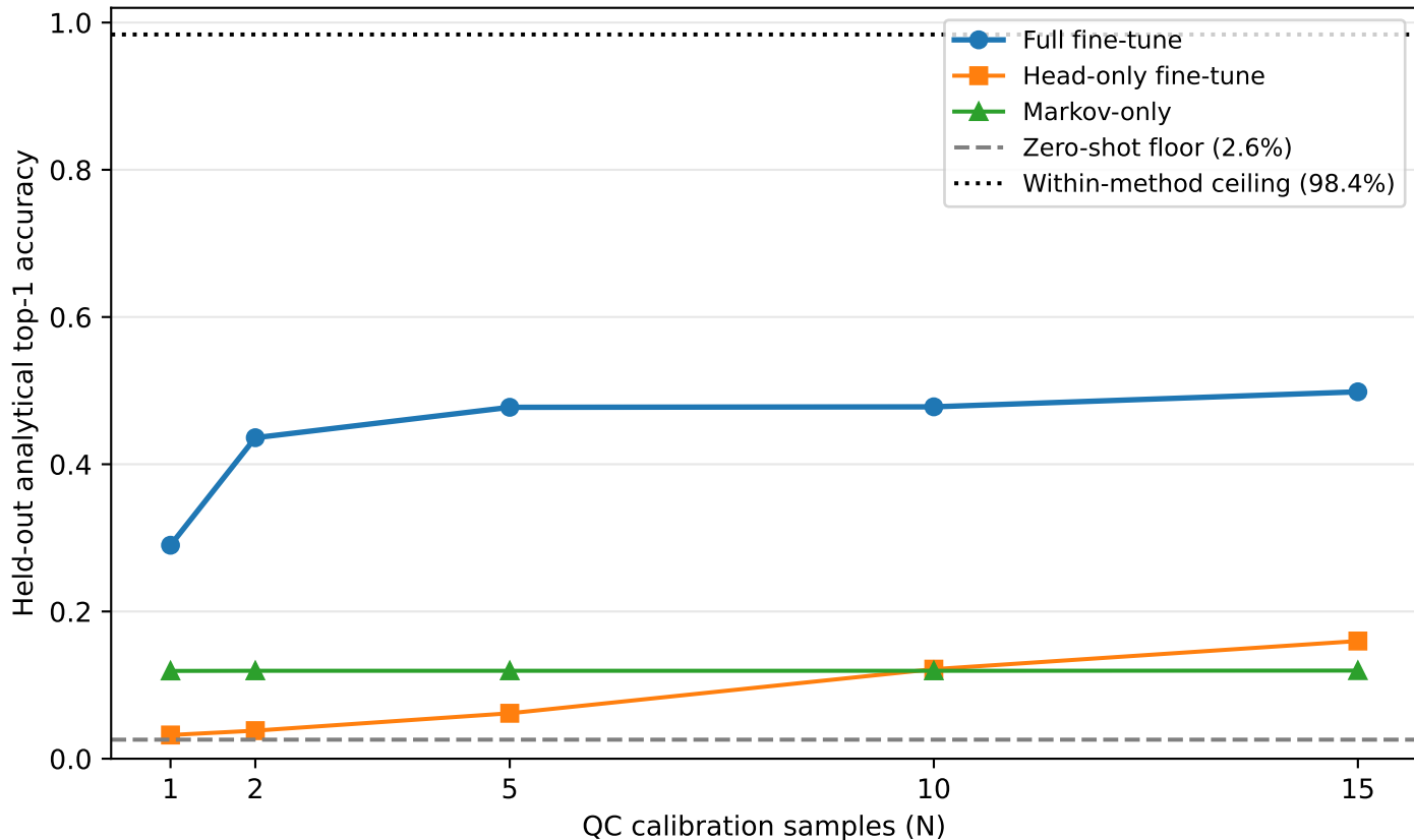
ST000990 transfer-learning recovery
