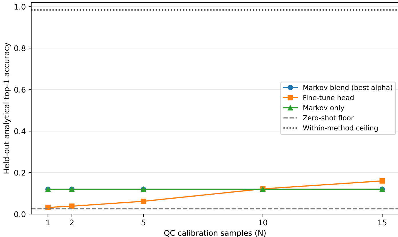
ST000990 few-shot transfer recovery
