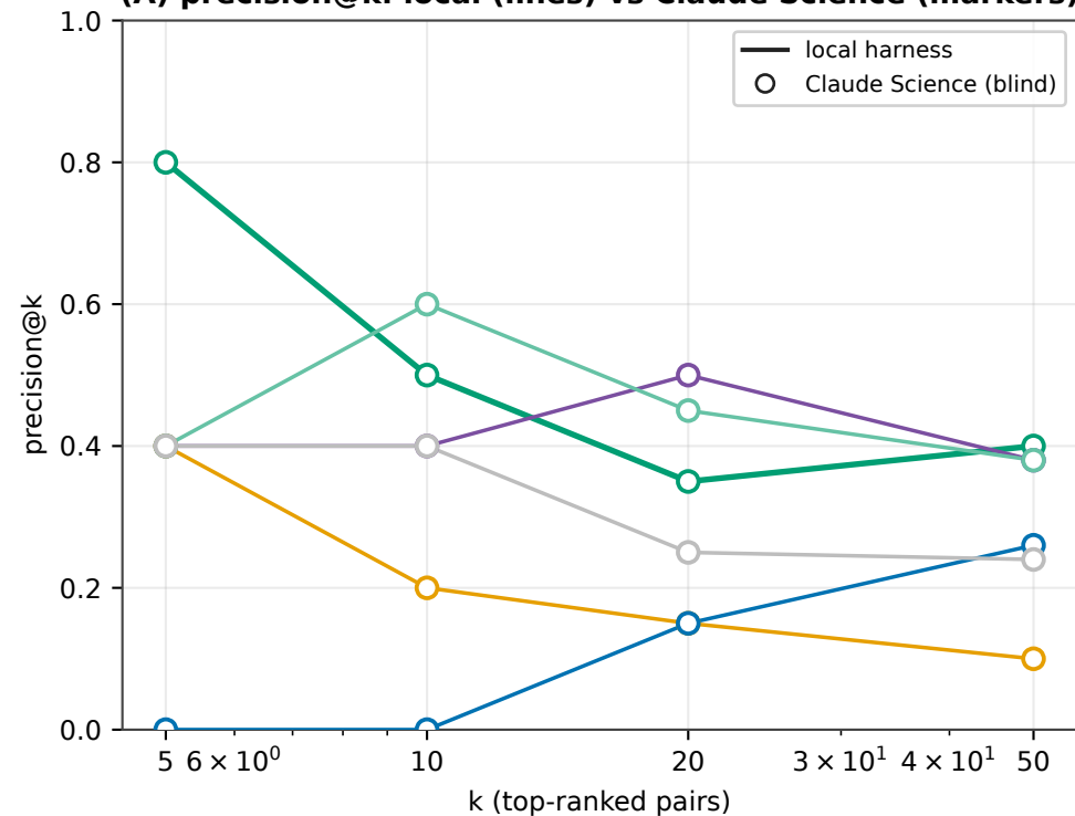
(A) precision@k: local (lines) vs Claude Science (markers)
