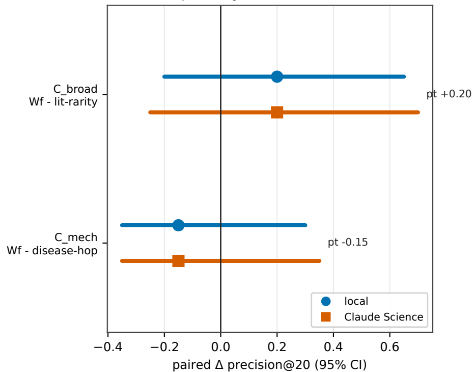
(B) co-primary contrasts: local vs CS
