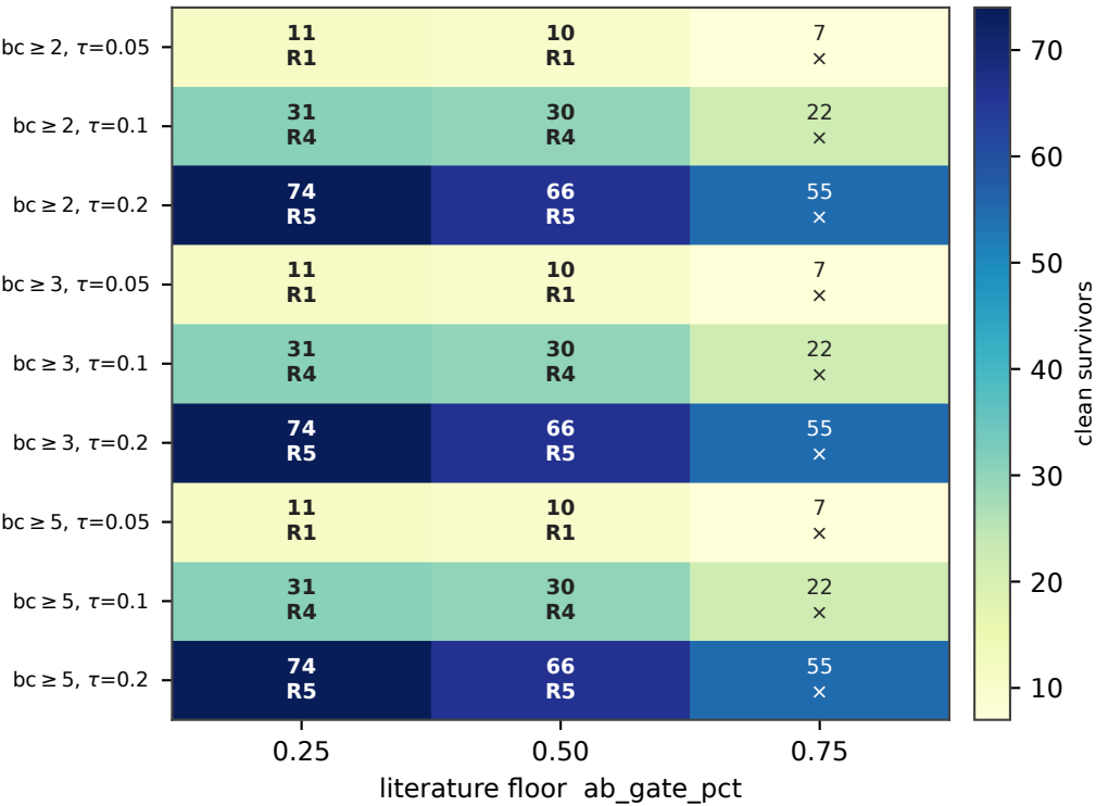
B. C10 gate grid -- clean survivors & NAB2 rank
