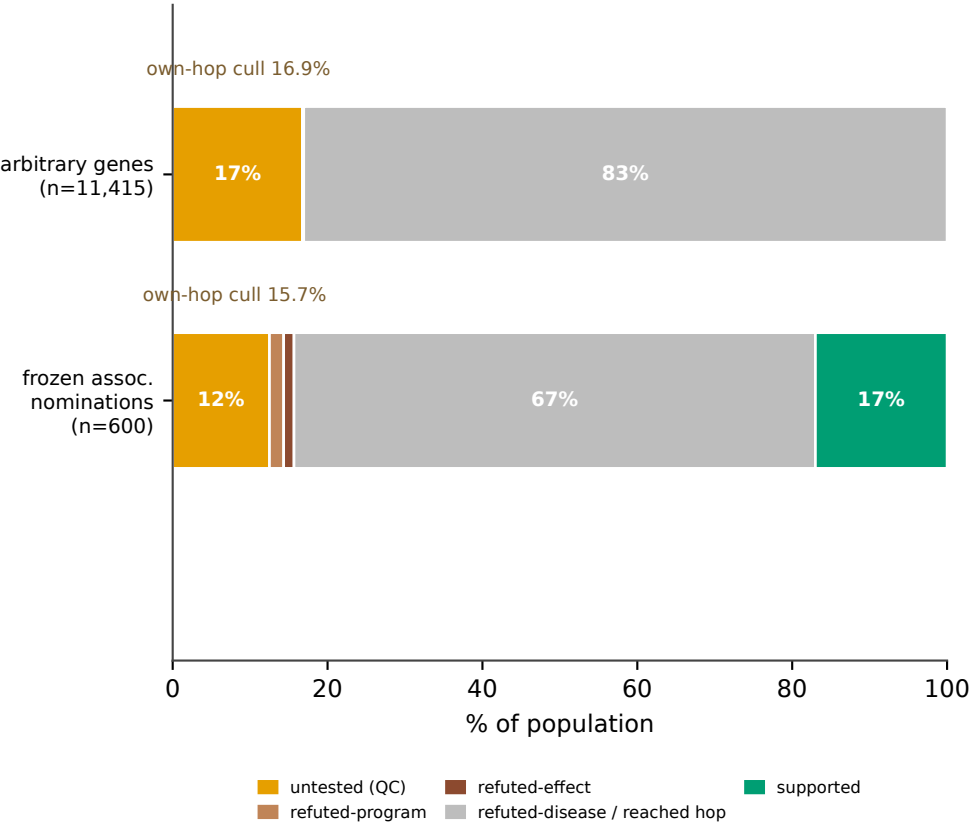
C. C2 -- the referee's own edge (out-of-funnel)
