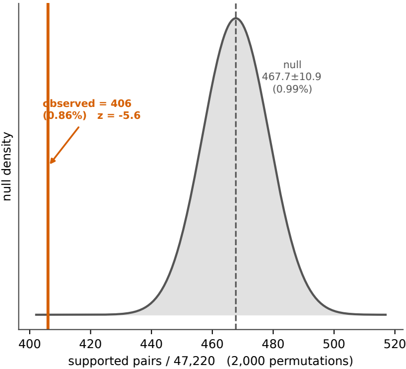
A. Control 2 -- disease-hop label-shuffle null
