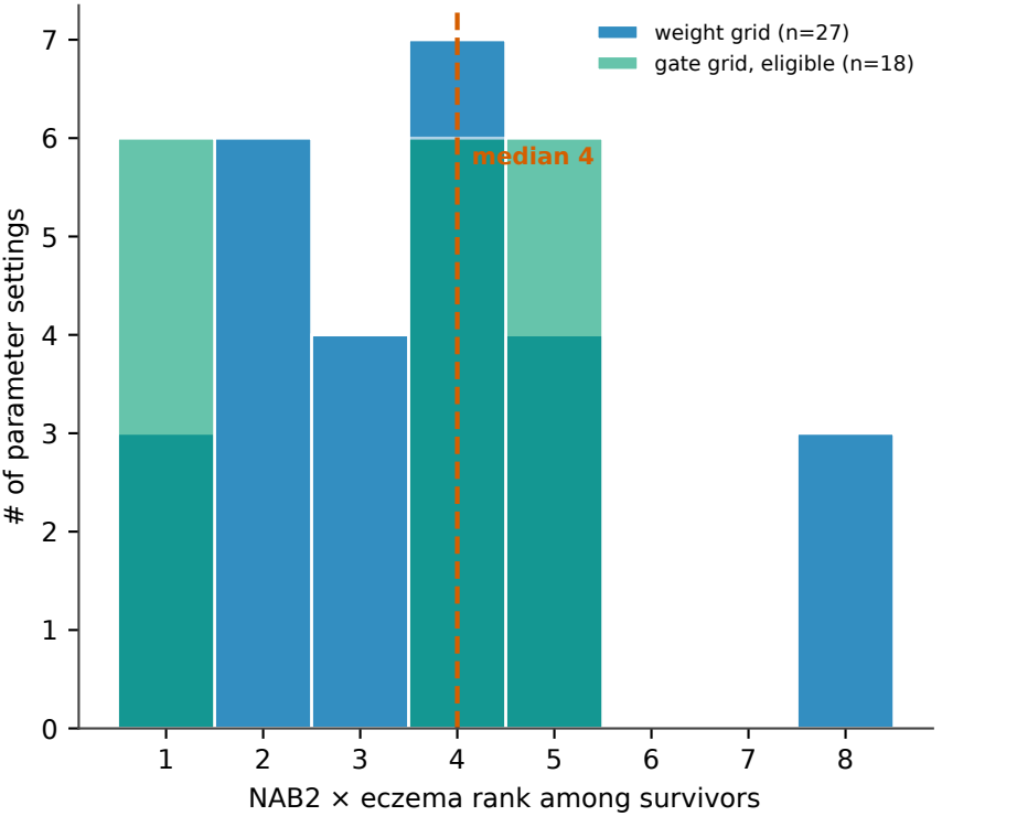
D. Control 3 -- flagship rank stability
