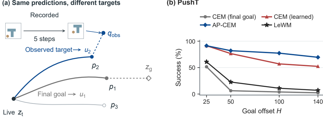
Figure 1: Changing the target improves control with the same frozen predictor. (a) Both target rules score the same endpoints p_i = F(z_t, u_i) . Final-goal scoring selects u_1 ; observed-target scoring selects u_2 . Solid curves show predictions; dashed segments show scoring distances. The target inset shows a recorded successor; positions and observations are schematic. (b) On PushT, intermediate targets sustain control as the recorded goal offset grows. Curves use paired standard-start queries and the same frozen LeWM weights.
