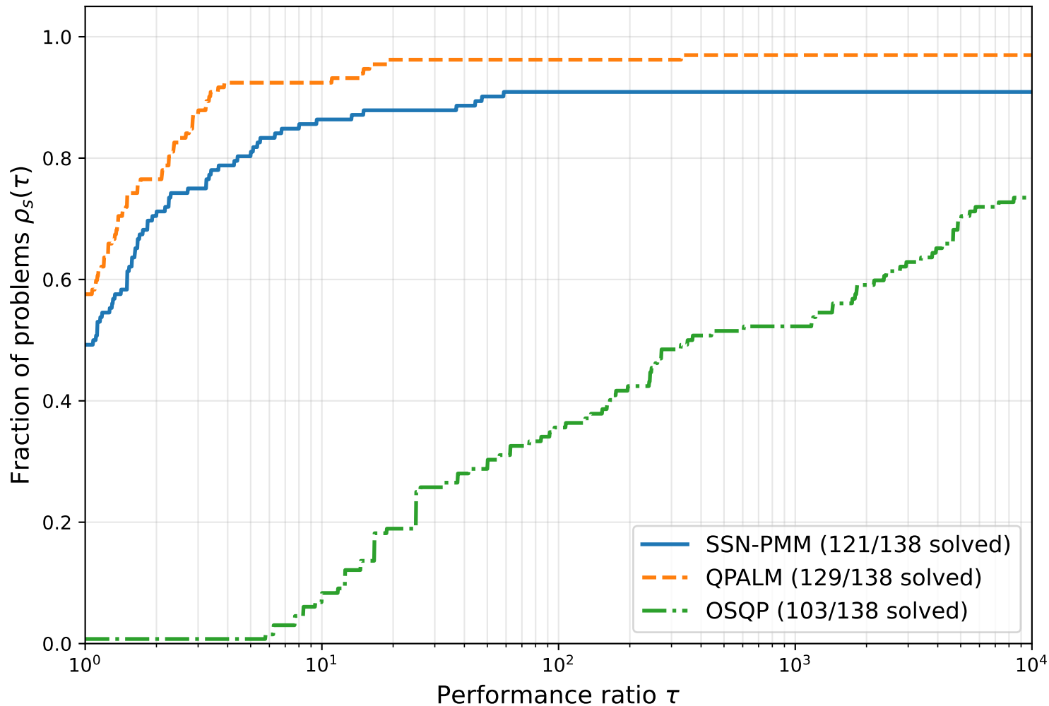
Performance profile — Maros-Meszaros QPs (iterations, tol = 10^{-6} , limit = 30 s)
