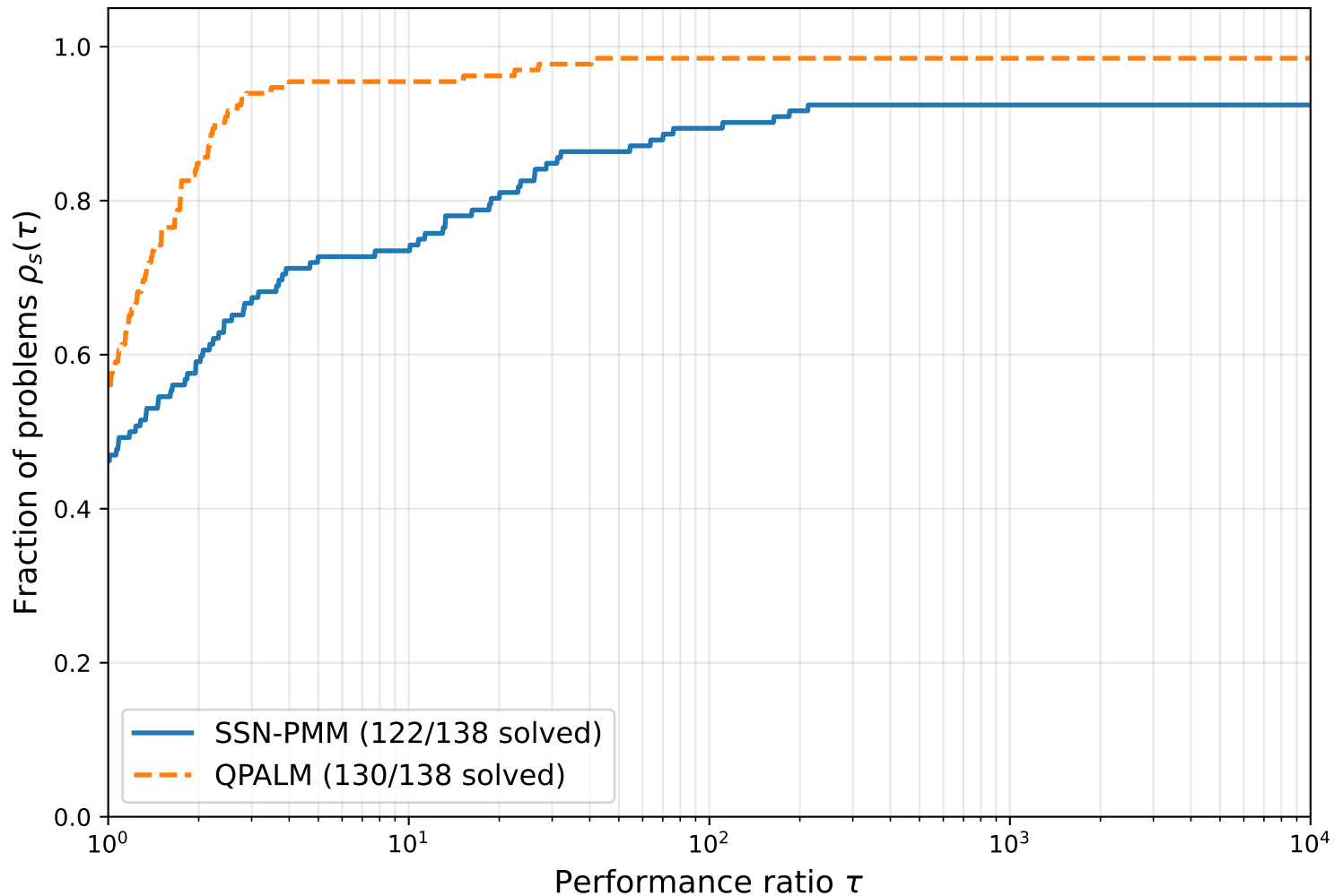
Performance profile — Maros-Meszaros QPs (inner iterations, tol = 10^{-6} , limit = 1 min)
