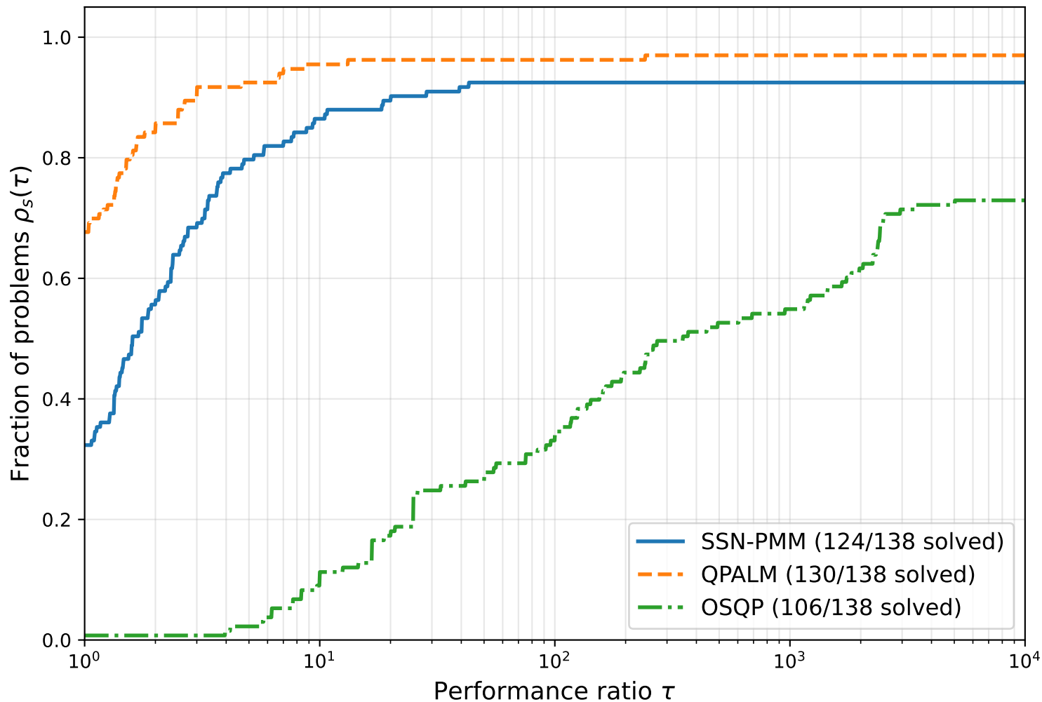
Performance profile — Maros-Mezzaros QPs (iterations, tol = 10^{-6} , limit = 1 min)
