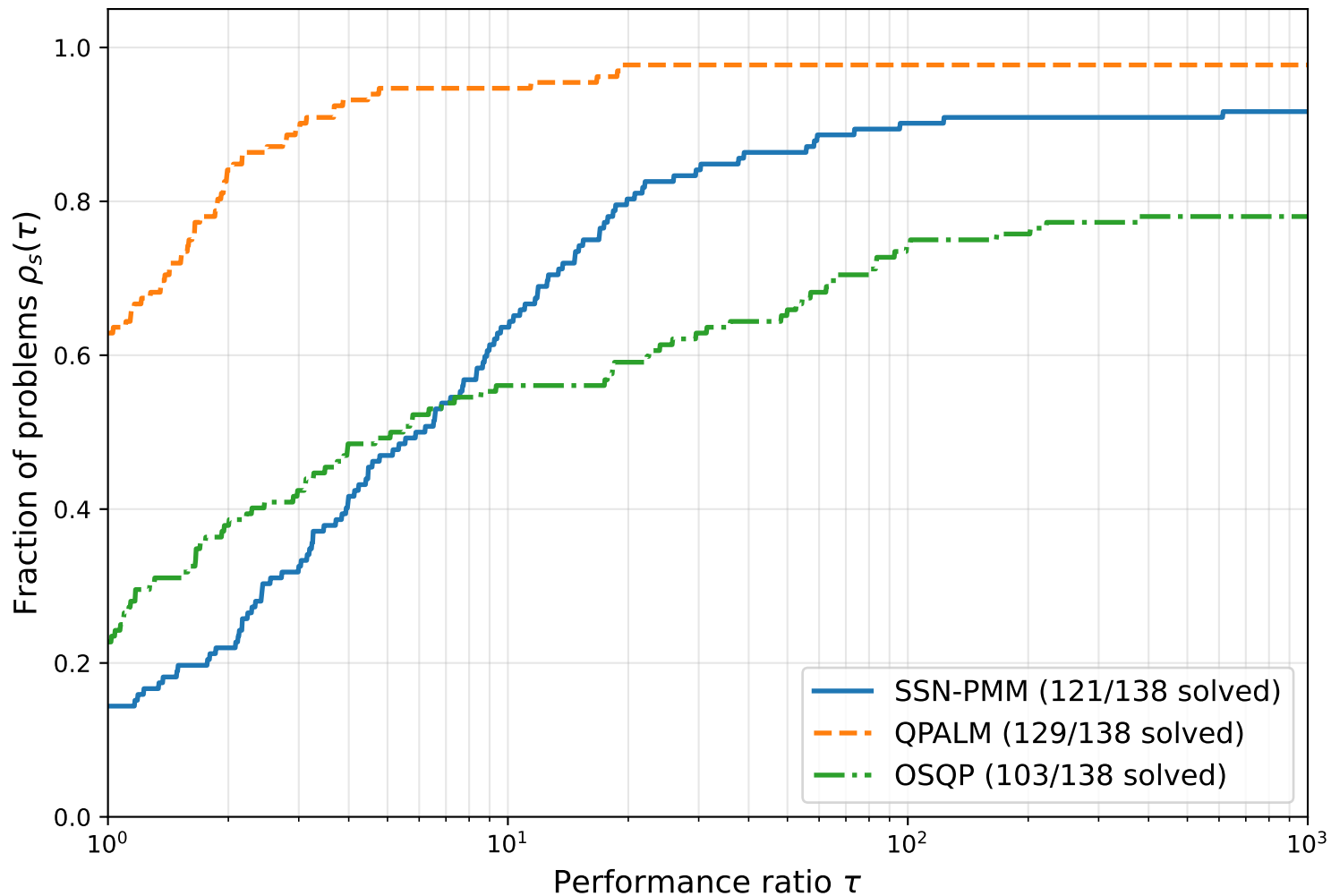
Performance profile — Maros-Meszaros QPs (solve time, \text{tol} = 10^{-6} , limit = 30 s)
