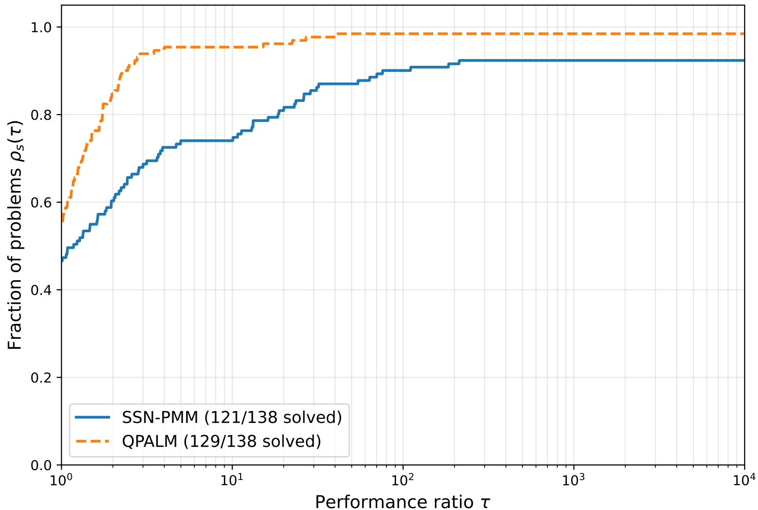
Performance profile — Maros-Meszaros QPs (inner iterations, tol = 10^{-6} , limit = 30 s)
