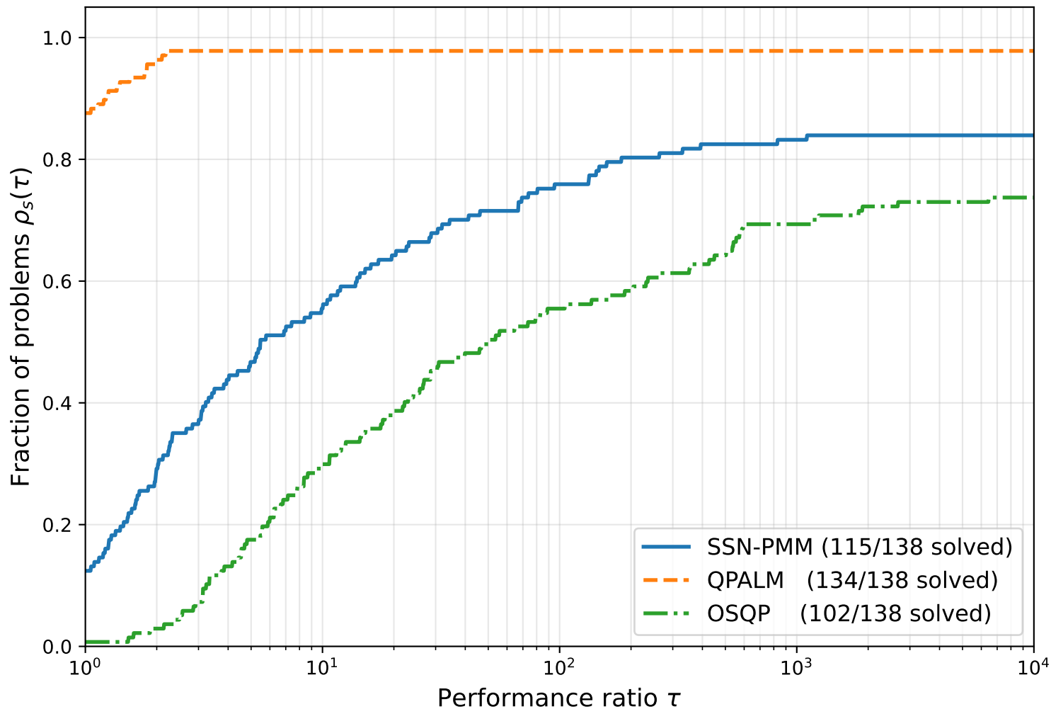
Performance profile — Maros-Meszaros QPs (iterations, tol = 10^{-6} , limit = 3 min)
