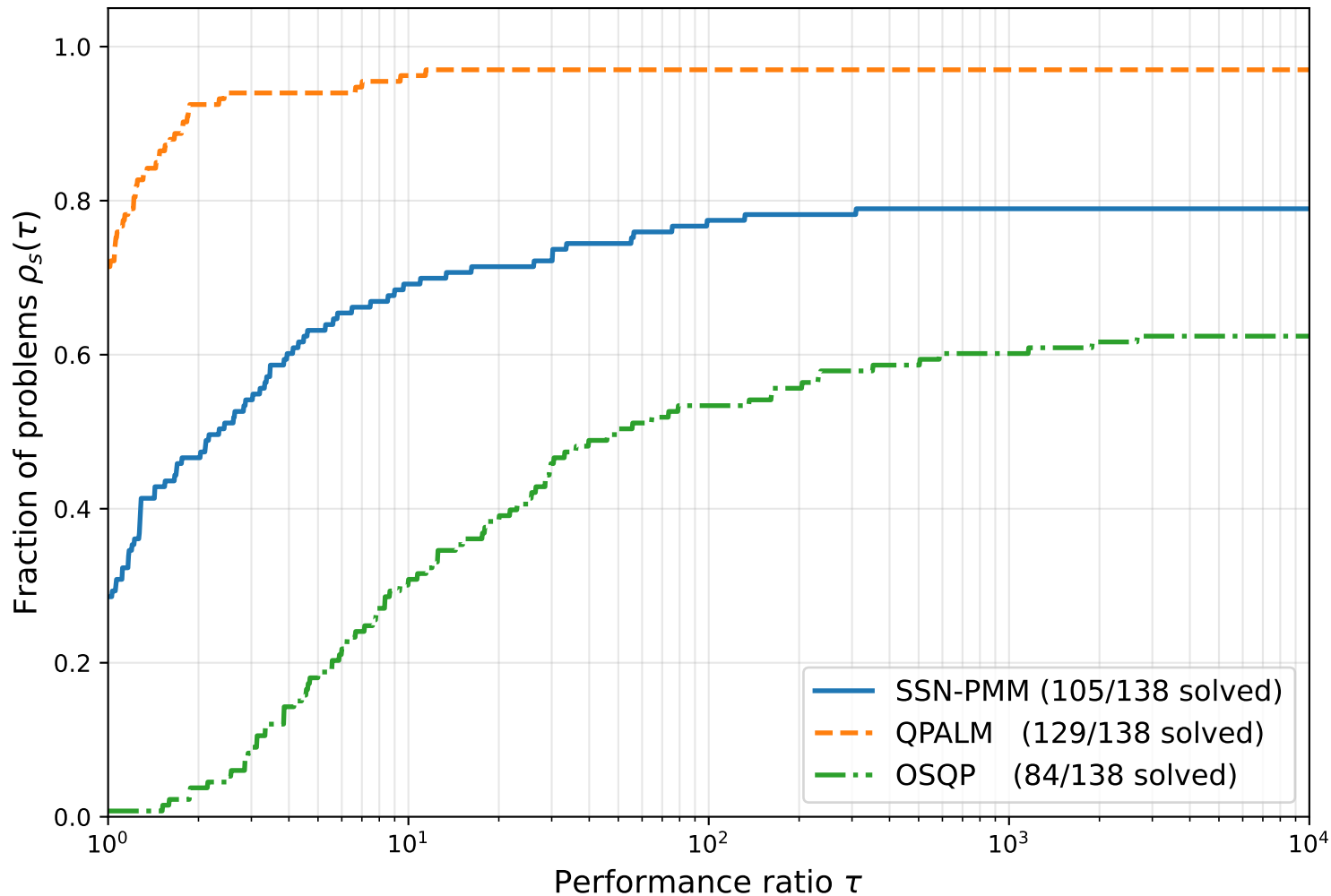
Performance profile — Maros-Meszaros QPs (iterations, tol = 10^{-6} , limit = 10 s)
