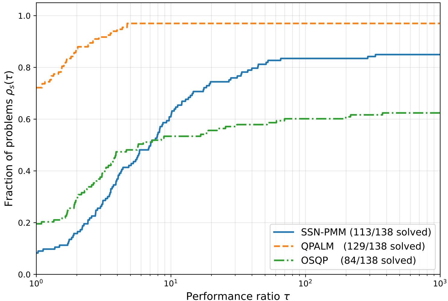
Performance profile — Maros-Meszaros QPs (solve time, \text{tol} = 10^{-6} , limit = 10 s)
