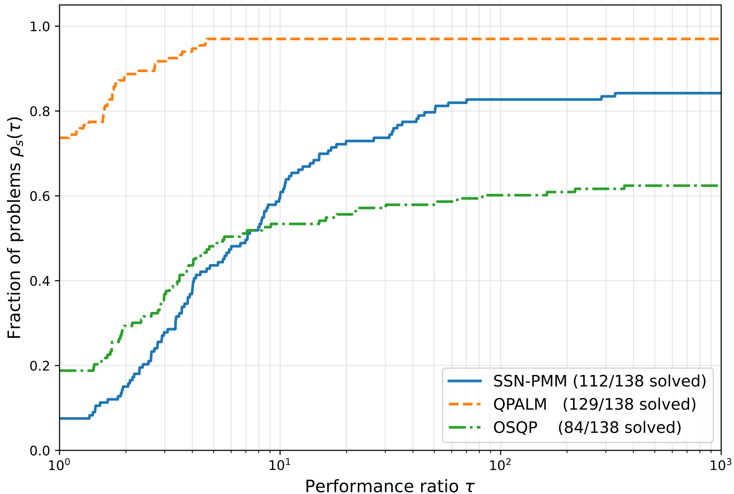
Performance profile — Maros-Meszaros QPs (solve time, tol = 10^{-6} , limit = 10 s)
