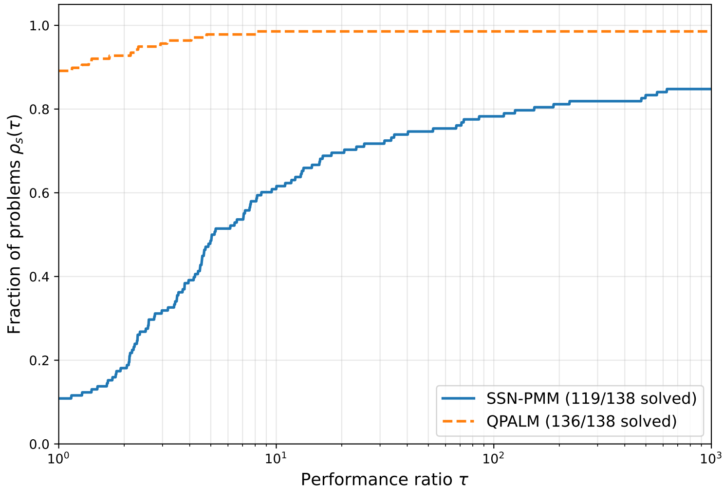
Performance profile — Maros-Meszaros QPs (solve time, tol = 10^{-6} , limit = 20 min)
