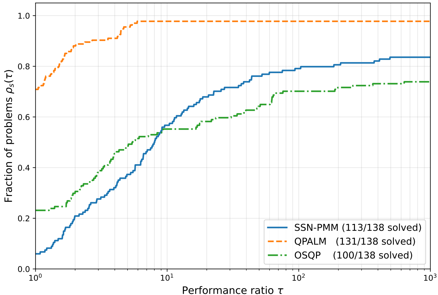
Performance profile — Maros-Mezzaros QPs (solve time, tol = 10^{-6} , limit = 1 min)
