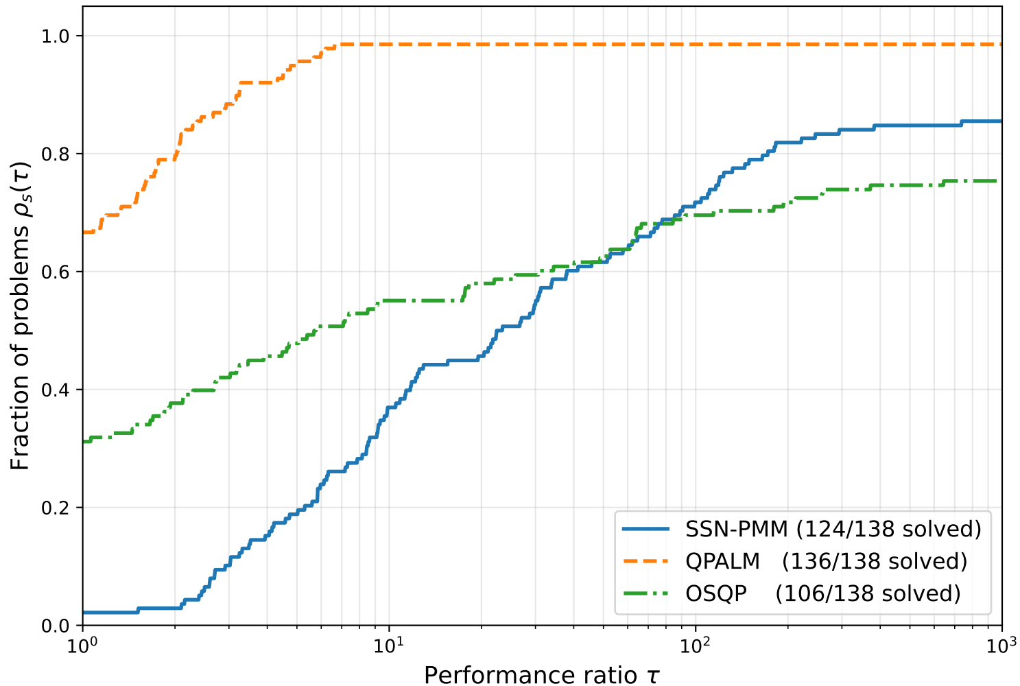
Performance profile — Maros-Meszaros QPs (solve time, tol = 10^{-6} , limit = 10 min)
