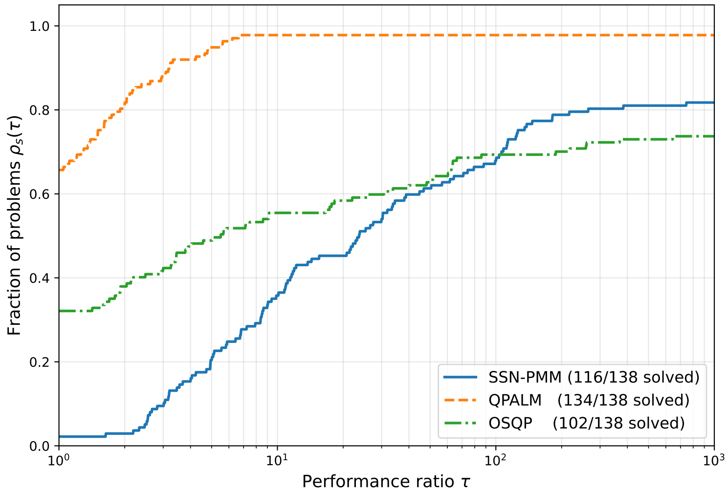
Performance profile — Maros-Meszaros QPs (solve time, tol = 10^{-6} , limit = 3 min)
