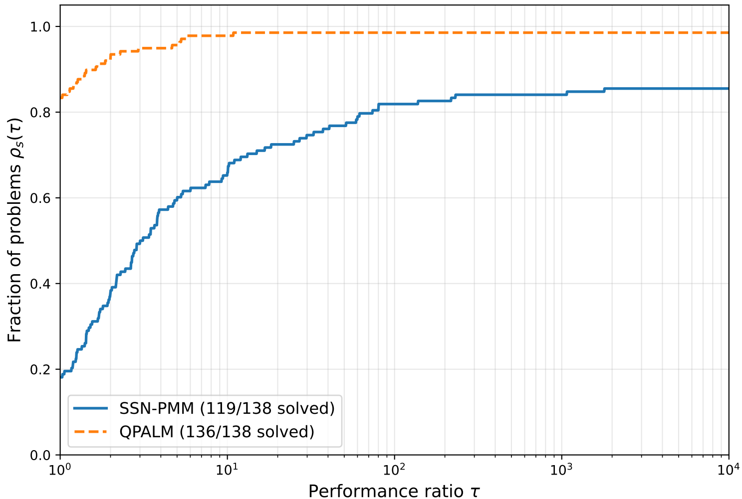
Performance profile — Maros-Meszaros QPs (iterations, tol = 10^{-6} , limit = 20 min)
