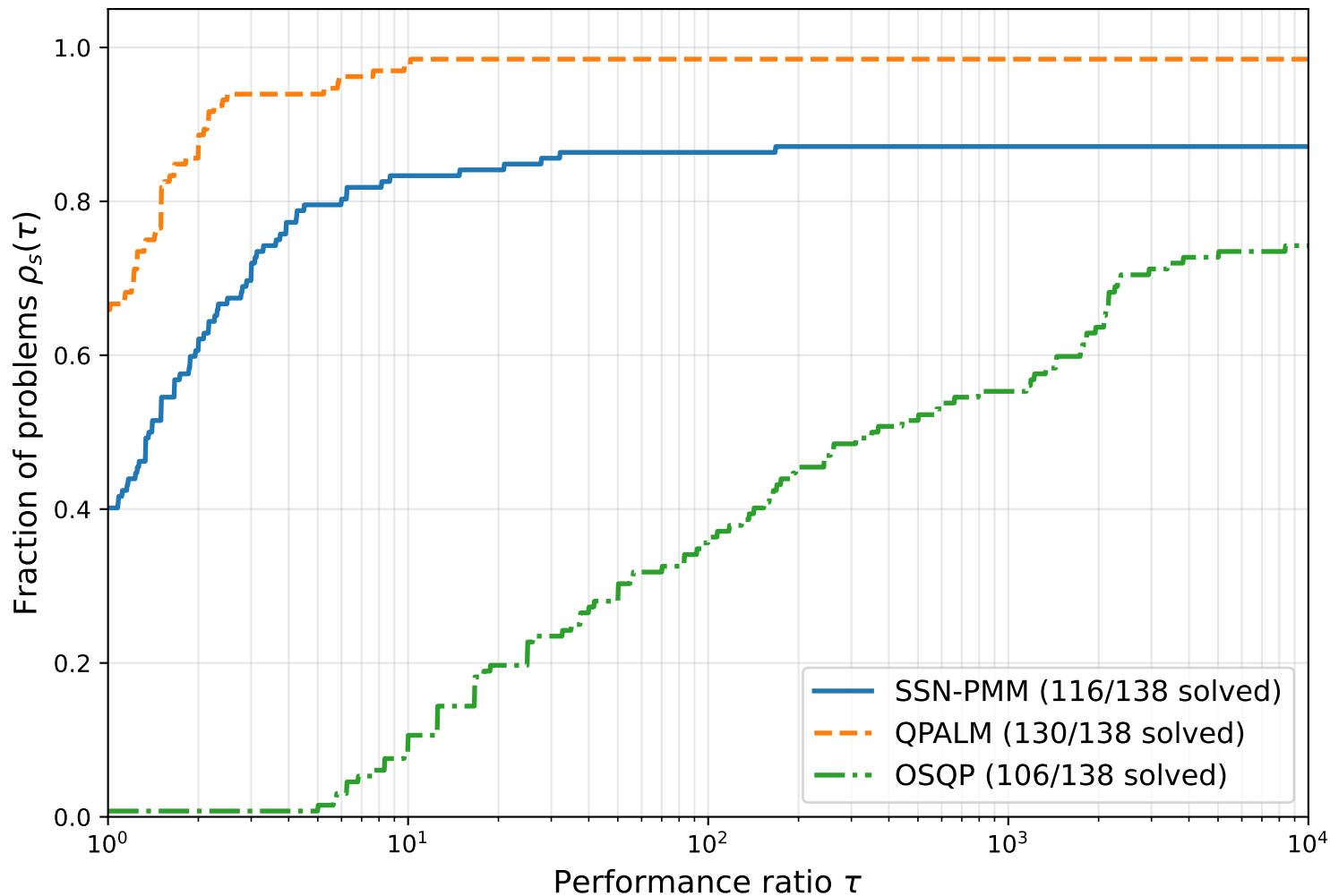
Performance profile — Maros-Meszaros QPs (iterations, tol = 10^{-6} , limit = 1 min)
