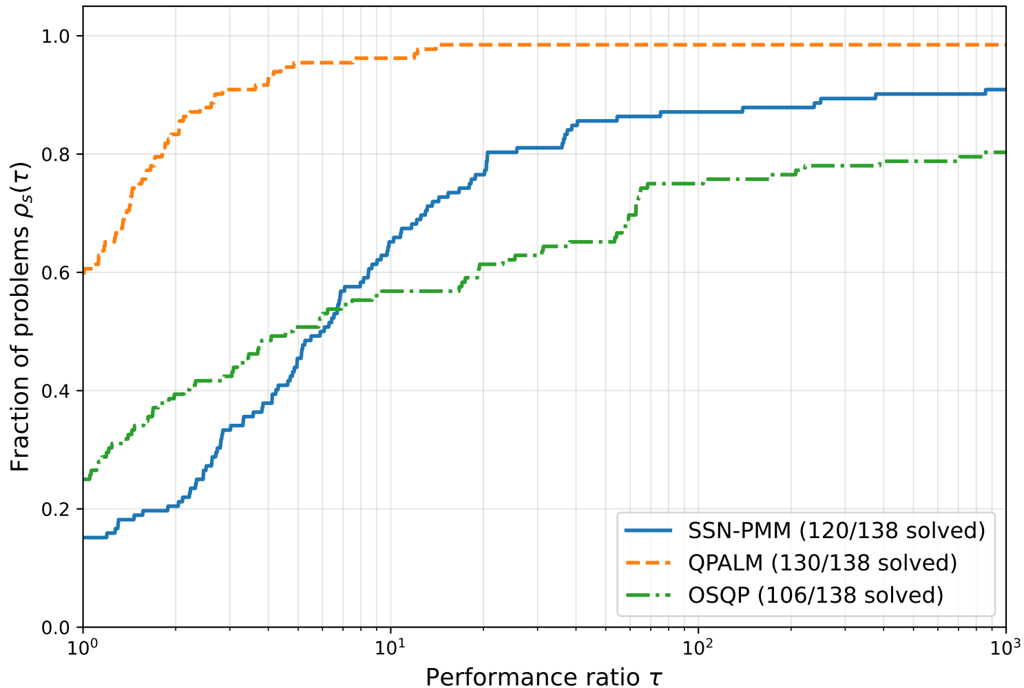
Performance profile — Maros-Meszaros QPs (solve time, tol = 10^{-6} , limit = 1 min)
