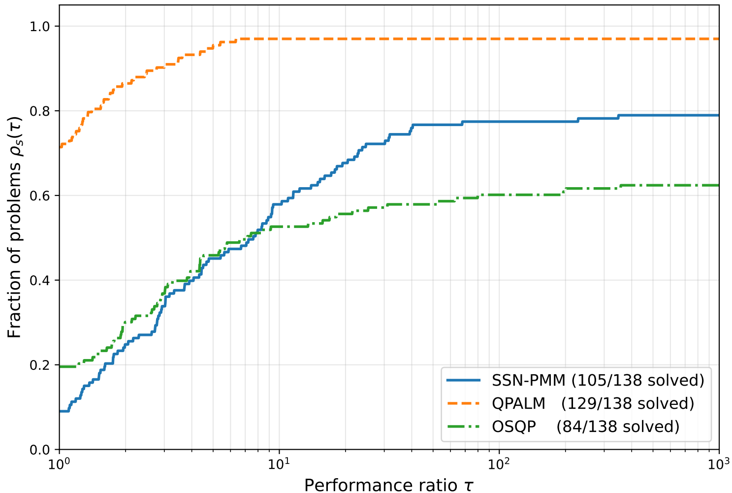
Performance profile — Maros-Mezzaros QPs (solve time, \text{tol} = 10^{-6} , limit = 10 s)
