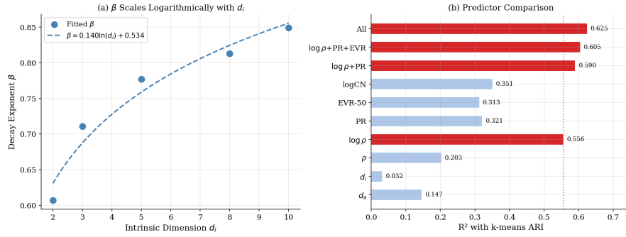
Fig. 4 (a) Decay exponent \beta scales logarithmically with d_i . (b) \log(\rho) achieves the highest R^2 among individual predictors, outperforming participation ratio and explained variance ratio.
