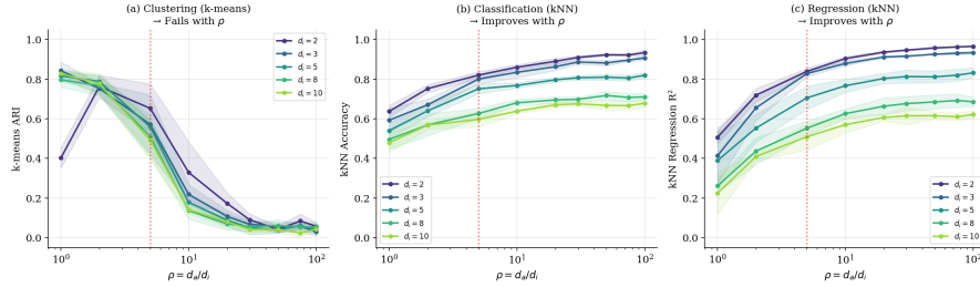
Fig. 2 Algorithm-dependent effects of \rho . k -means degrades (left) while k NN classification (center) and regression (right) improve. This divergence reveals a geometric tradeoff rather than a simple curse.
