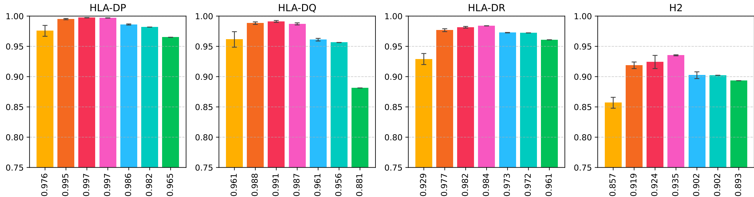
Mass Spectrometry
