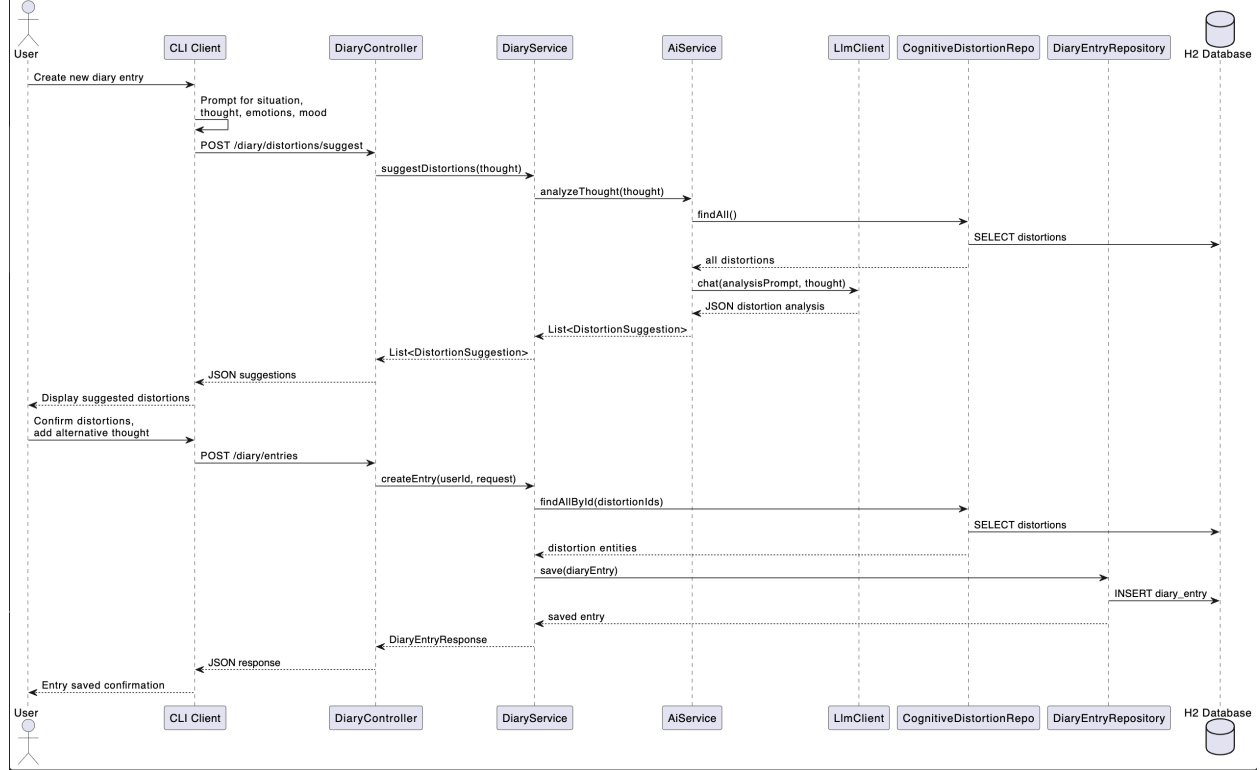
Sequence Diagram - Diary Entry with AI Analysis
