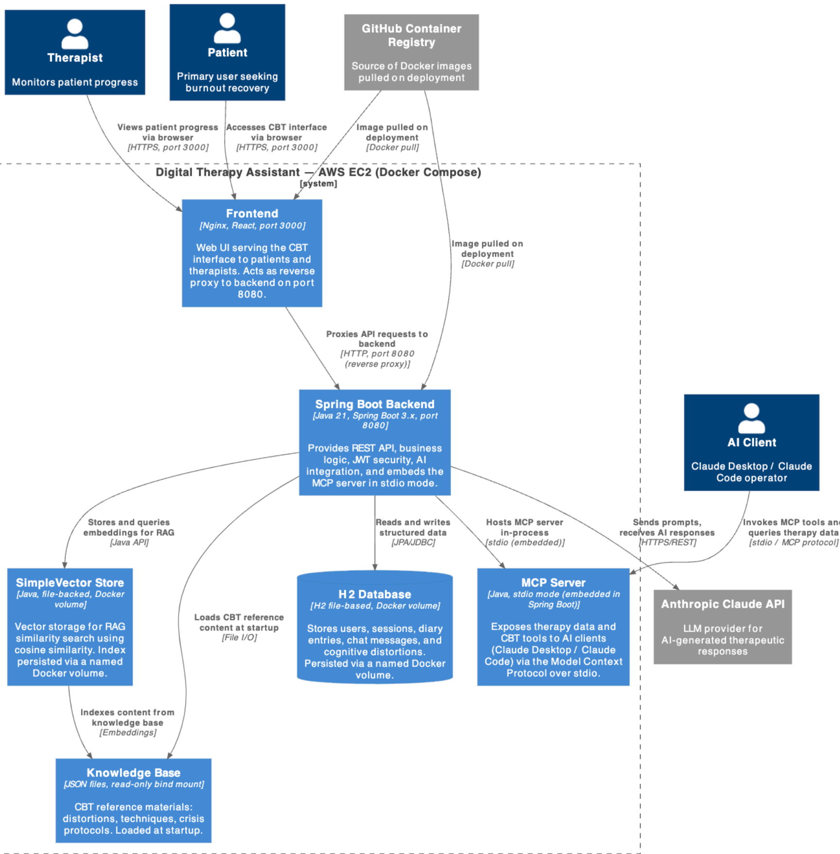
Container Diagram - Digital Therapy Assistant (Updated)
