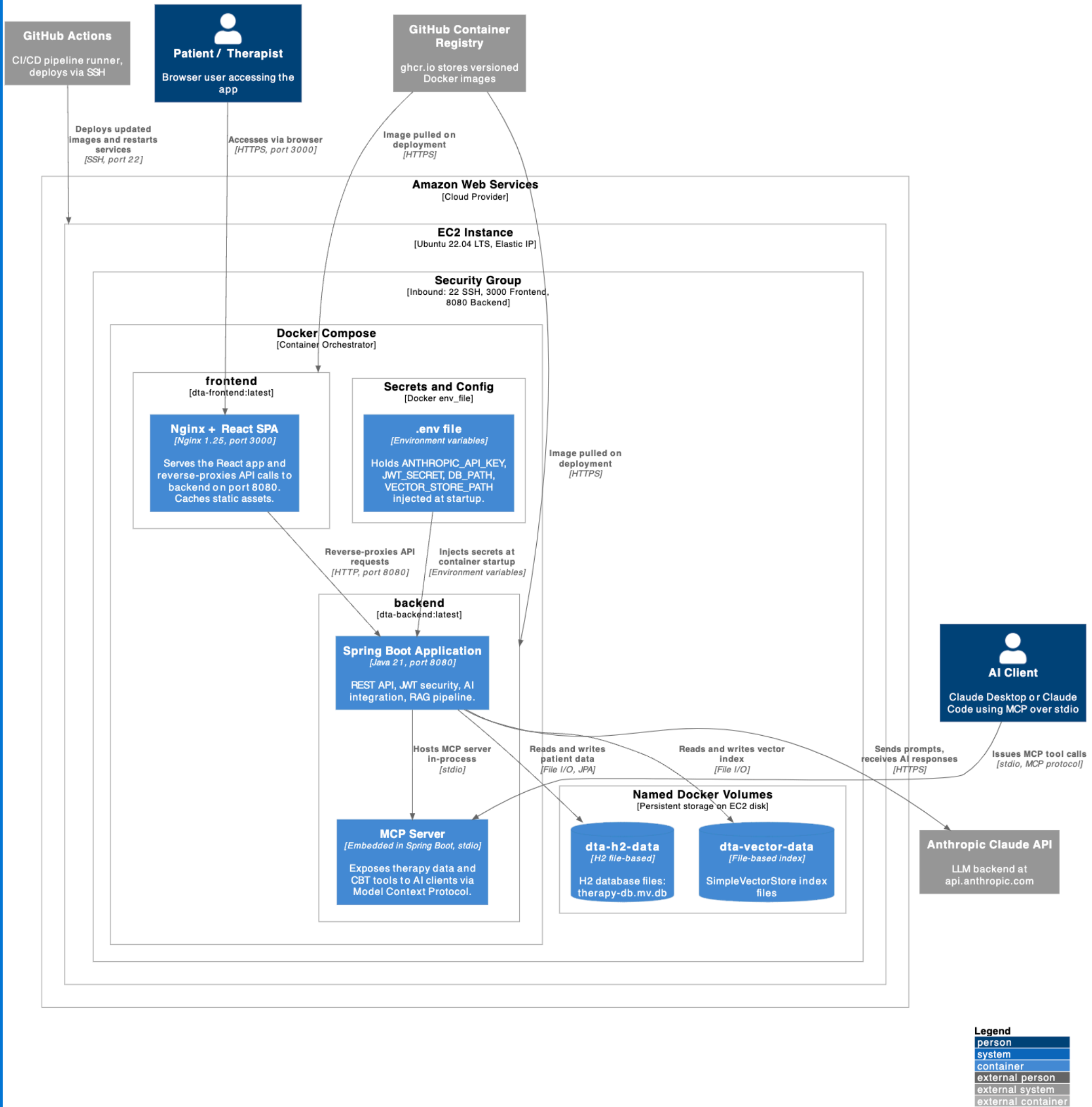
Deployment Diagram - Digital Therapy Assistant on AWS EC2
