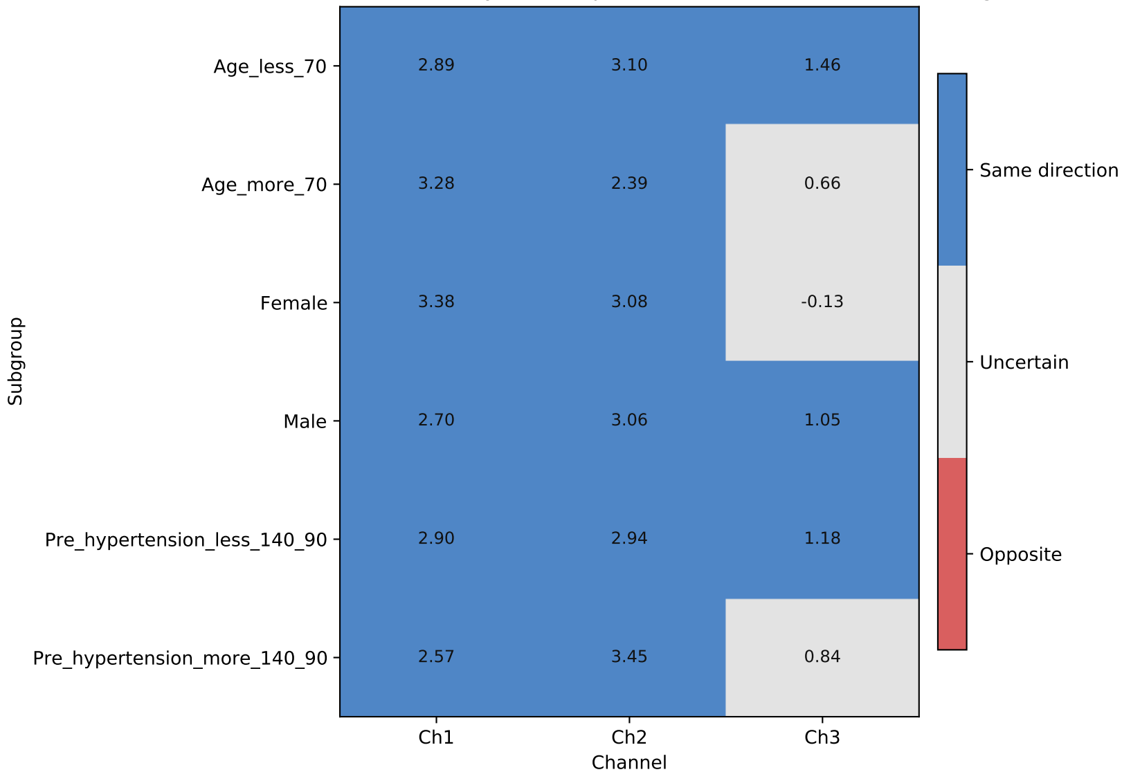
Direction Consistency Heatmap (value = Delta rSO2 for +5 mmHg)
