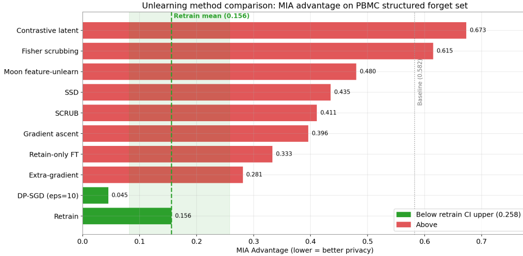
Figure 5: MIA advantage by method on PBMC-33k structured forget set ( n = 30 ). The dashed line marks the 5-seed retrain advantage mean (0.156) with shaded nested 95% CI [0.082, 0.258]. DP-SGD’s advantage (0.045) is not distinguishable from retrain but trains from scratch. No post-hoc unlearning method’s advantage-difference CI reaches zero.
