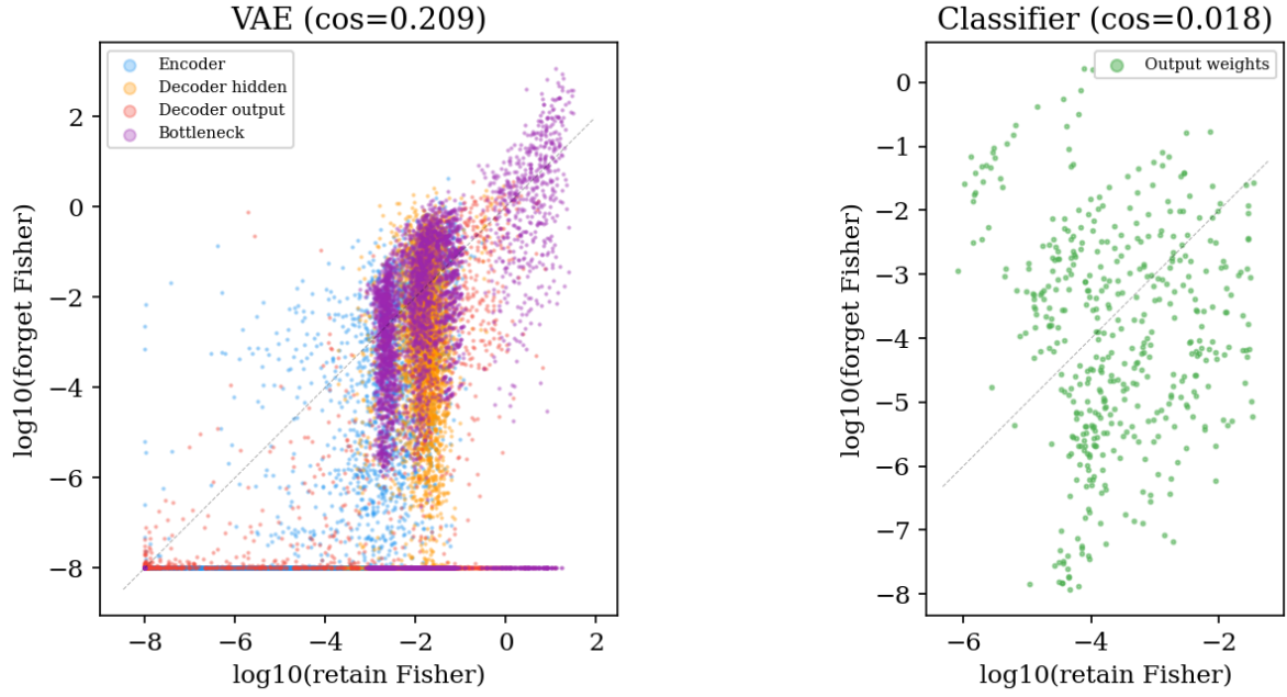
Figure 6: Per-parameter Fisher magnitude (log scale) for forget vs. retain sets. Left: VAE parameters are correlated (log-Fisher r = 0.71 ), confirming that the same parameters matter for both sets. Right: classifier parameters show no correlation ( \cos = 0.018 ), with forget-set Fisher concentrated in a few class-specific weights.
