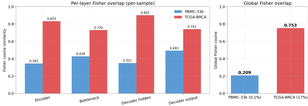
Figure 3: Fisher overlap on PBMC-33k (0.1% forget fraction) versus TCGA-BRCA (17%). Left: per-layer cosine. Right: global cosine. TCGA-BRCA overlap is uniformly higher, driven by the larger forget fraction and fewer output dimensions.
