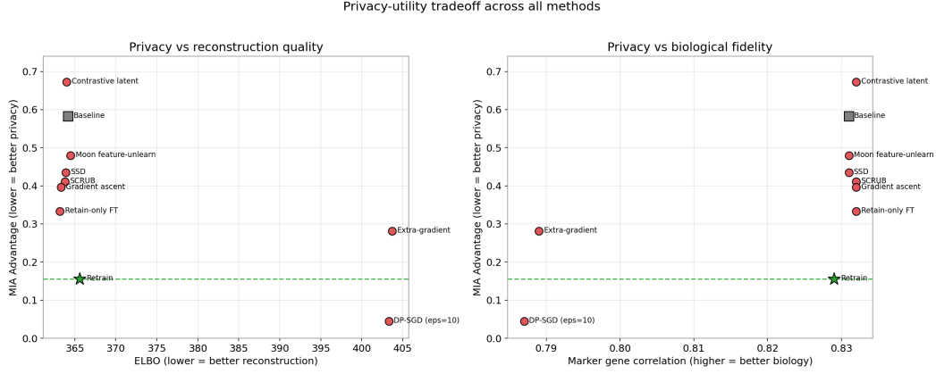
Figure 4: Privacy-utility tradeoff across all methods. Left: advantage vs. ELBO. Right: advantage vs. marker gene correlation. Methods that preserve utility (upper cluster) fail on privacy; methods that reduce advantage (DP-SGD, extra-gradient) pay a utility cost. Only retrain achieves both.
