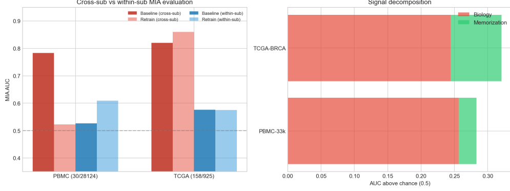
Figure 1: Biology confound across datasets. Left: cross-subtype vs. within-subtype MIA AUC for PBMC and TCGA-BRCA. With within-subtype matching, baseline and retrain AUCs converge. Right: decomposition of the cross-subtype AUC signal into biology (red) and memorization (green) components.
