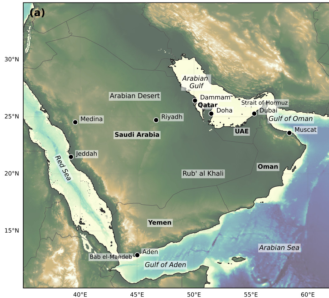
Arabian Peninsula
