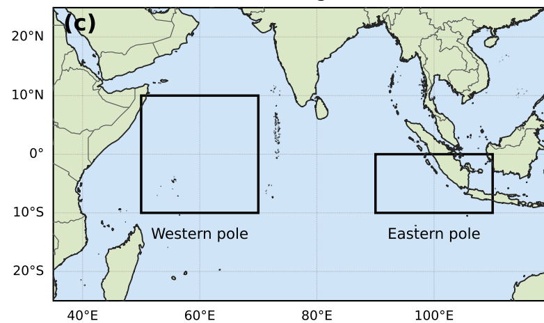
IOD Region
