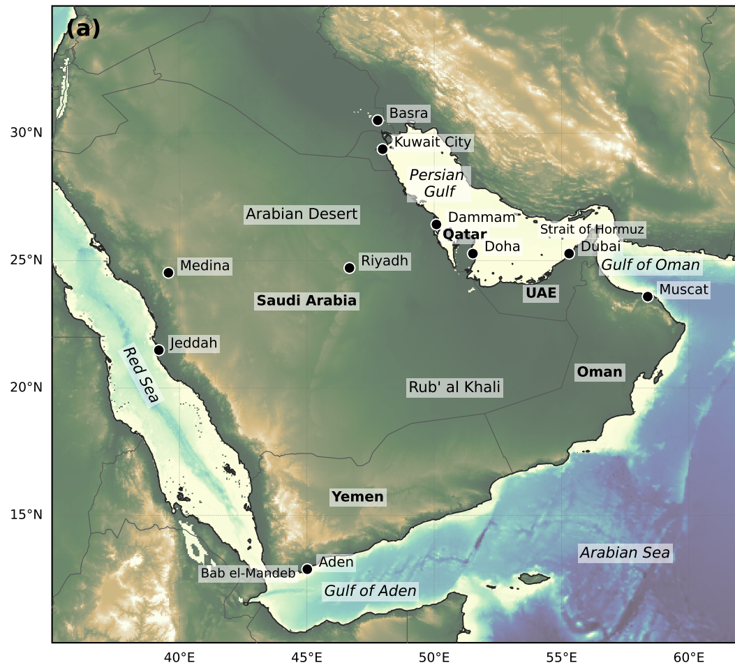
Arabian Peninsula
