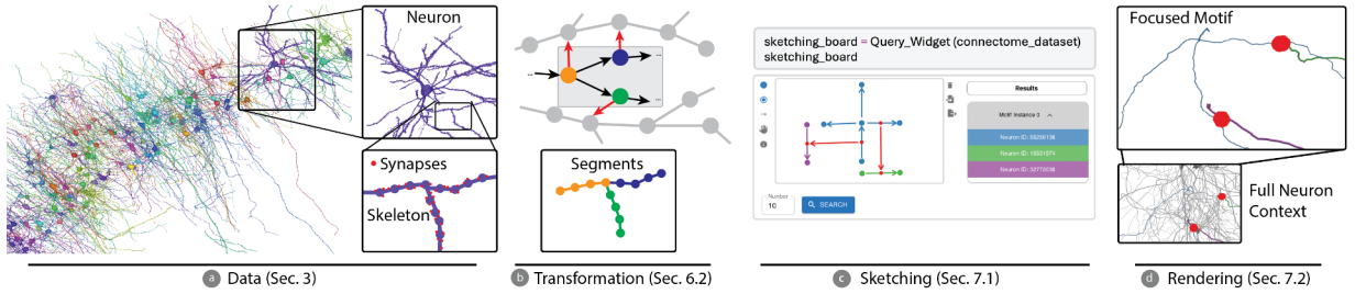
Fig. 3: MoMo Workflow. (a) Given a connectome dataset, we (b) transform the respective neurons and synapses into our neuron morphology-aware graph representation. Each node in the graph depicts a neuron segment that is connected to other segments through synaptic connections (red arrows) or to neighboring segments (black arrows). (c) The transformed dataset is interactively queried by sketching motifs. (d) Finally, users can explore identified motif instances in interactive 3D renderings and highlight the motif's morphology through a focus & context approach. Data: Human temporal cortex / H01 [60] (a), MICrONS [4] (d).
