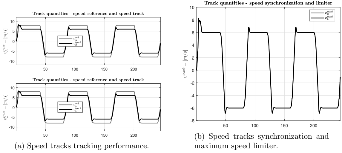
Figure 6.12: Simulation results scenario 1.
