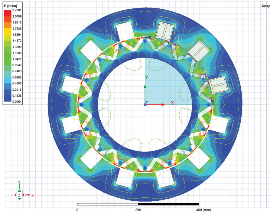
Figure 8.12: Magnetostatic analysis.
