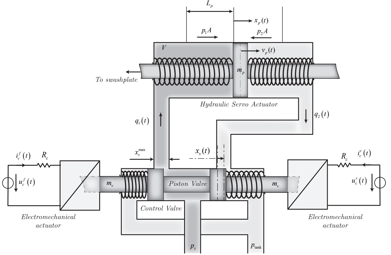
Figure 4.1: Swash-plate actuator.
