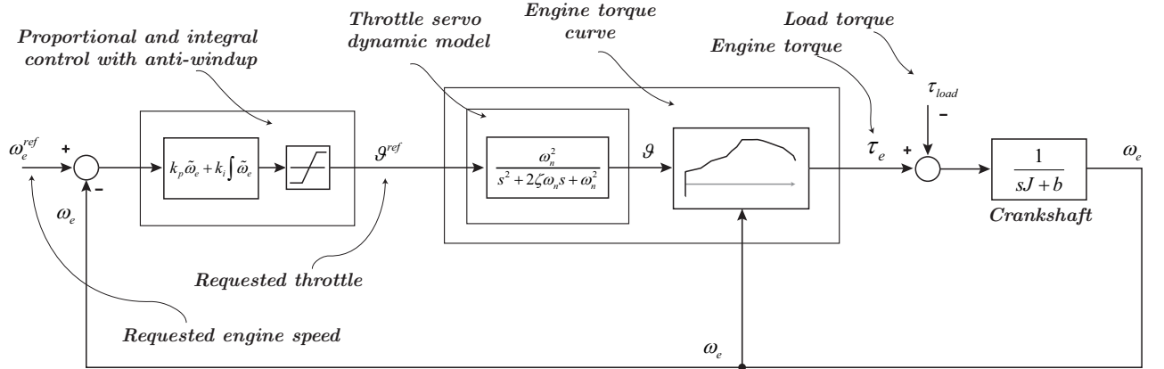
Figure 5.2: Engine model and control architecture.
