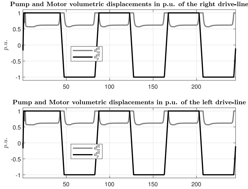
Figure 6.21: Volumetric displacements.
