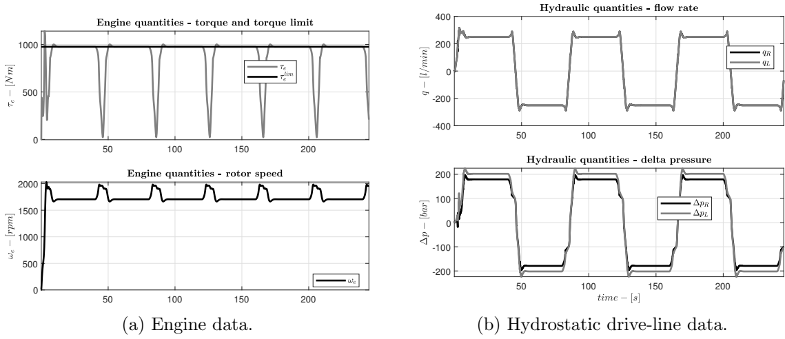
Figure 6.11: Simulation results scenario 1.
