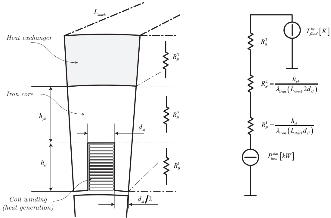
(b) Equivalent steady-state thermal circuit.
