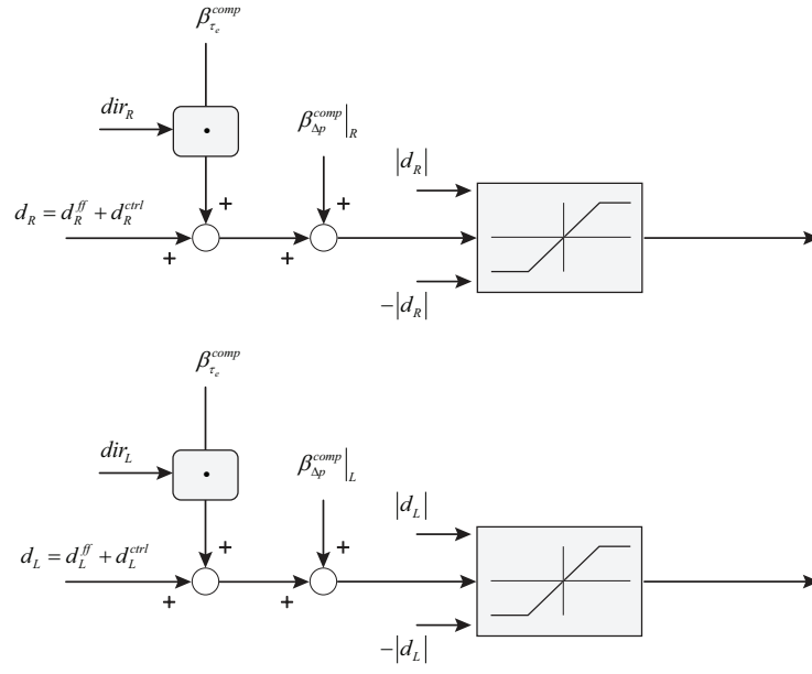
Figure 6.7: Global volumetric displacement construction comprehensives of the compensations.
