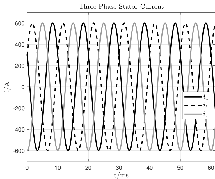
Figure 11.2: Simulation results: stator currents.
