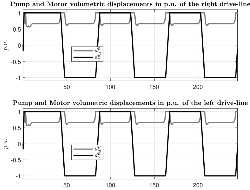
Figure 6.13: Volumetric displacements.
