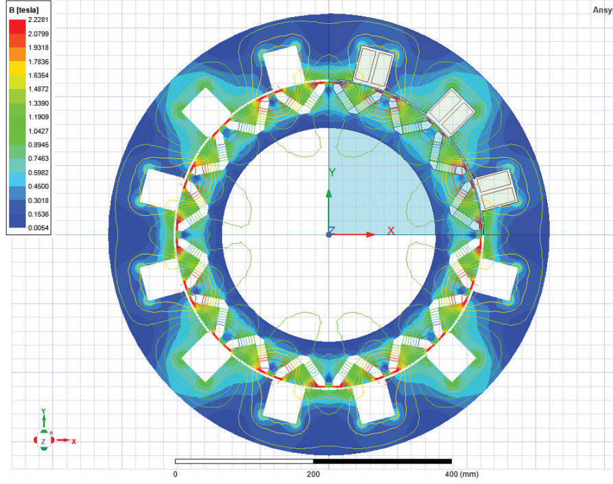
Figure 8.6: Magnetostatic analysis.
