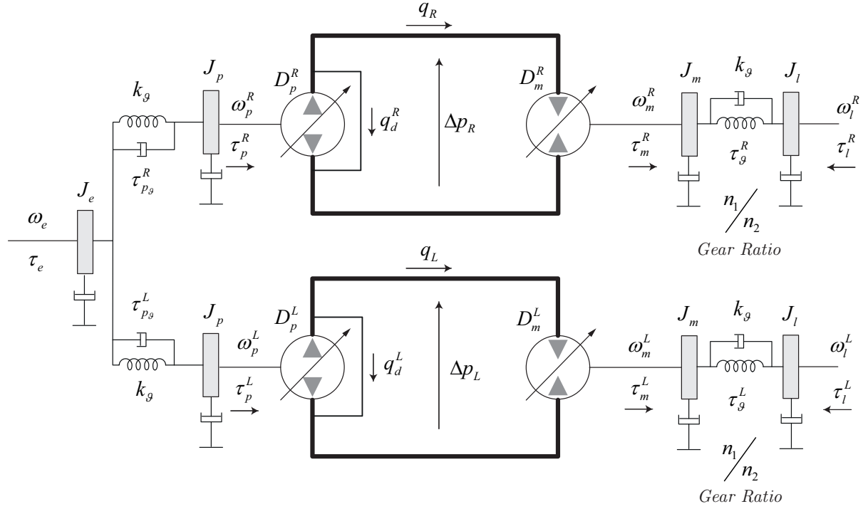
Figure 2.1: Hydrostatic transmission - the whole transmission power-train is made two, independent lines, one for the left side ( L ) and one for the right side ( R ) as follows.
