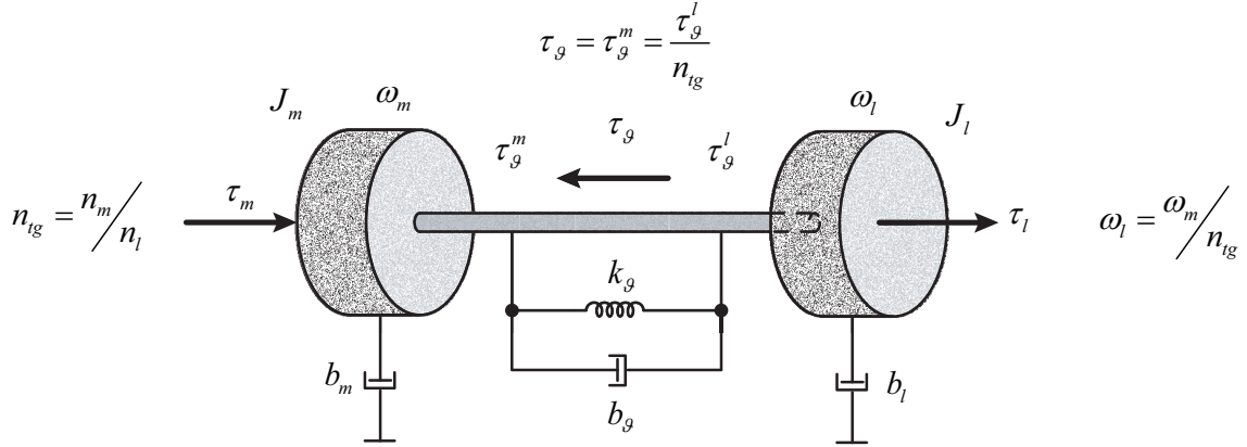
Figure 3.2: Drive-gear representation as flexible shaft model.
