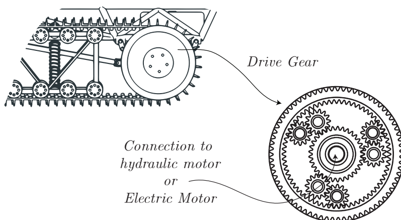
Figure 3.1: Drive-gear representation.
