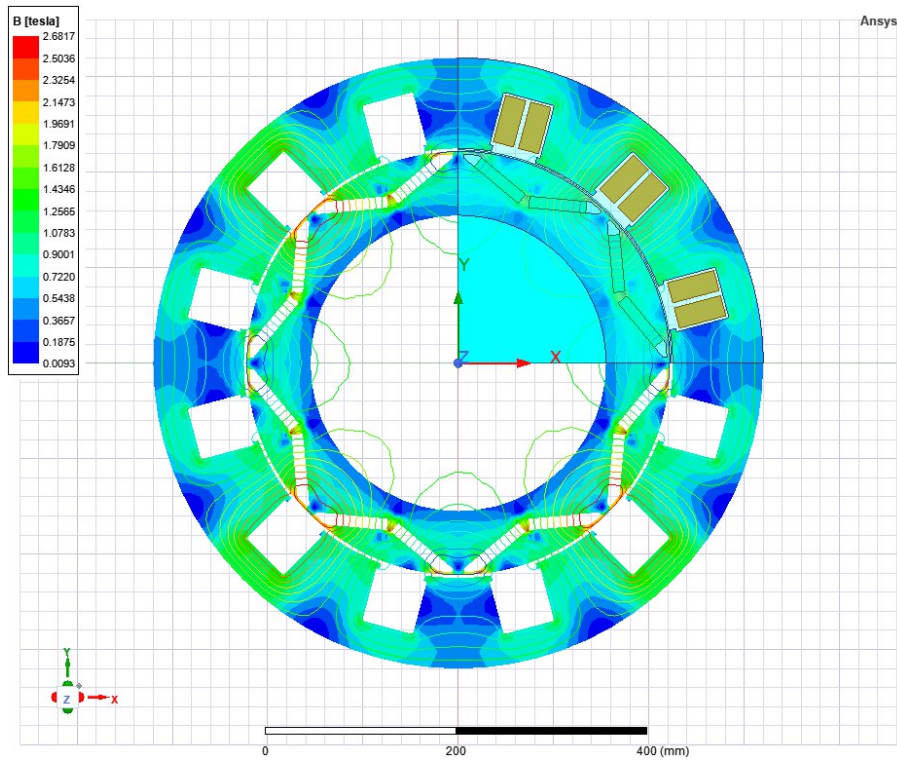
Figure 8.9: Magnetostatic Analysis.
