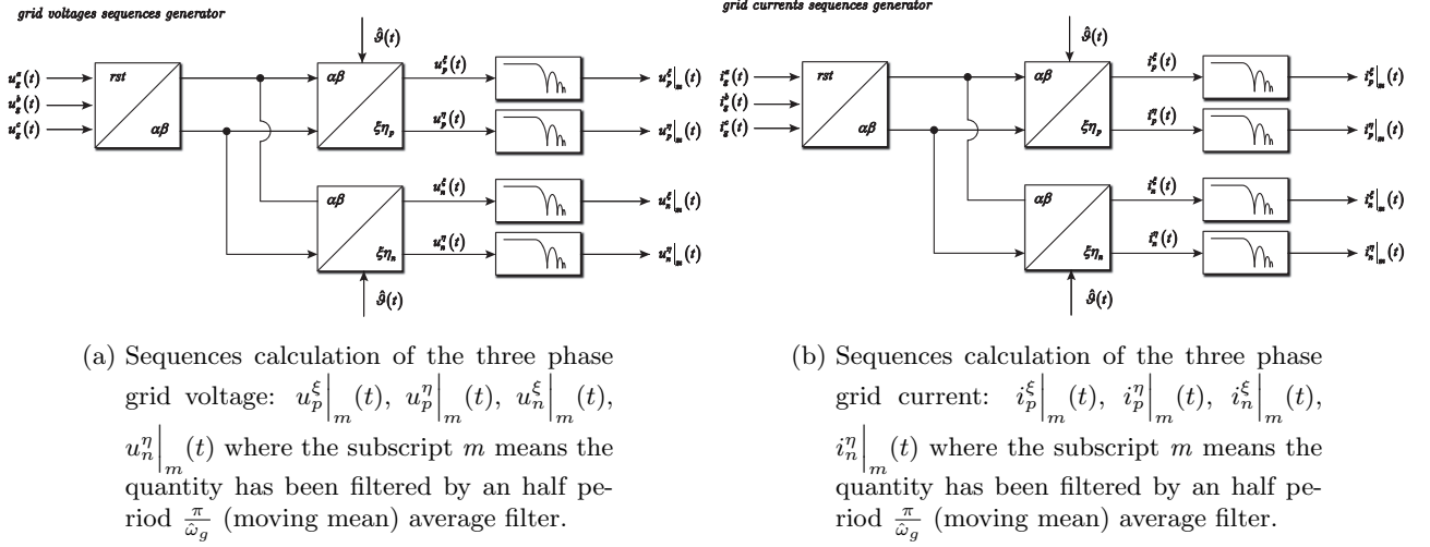
Figure 47: Grid voltage and current sequences calculation.
