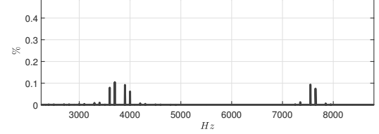
Four modules - grid phase current spectrum 50 \leq h \leq 160 at rated operating point - I_{cc} = 50kA
