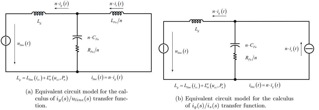
Figure 11: Equivalent circuit model (per phase equivalent star connection) of the grid/transformer/output-filter/AFE-VSI system for the case of n -parallelised ElectricalDrive . Equivalent circuit for the calculus of i_g(s)/u_{line}(s) transfer function (a), and equivalent circuit for the calculus of i_g(s)/i_s(s) transfer function (b).
