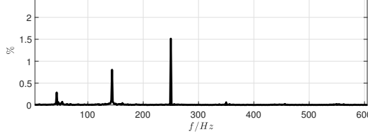
Eight modules - grid phase current spectrum 2 \leq h \leq 11 at rated operating point - I_{cc} = 50 \text{ kA}
