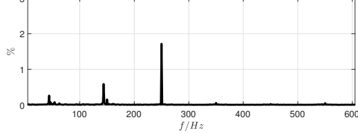
Eight modules - grid phase current spectrum 2 \leq h \leq 11 at rated operating point - I_{ce} = 50kA
