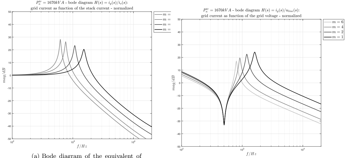
(b) Bode diagram of the equivalent of the transfer function: i_g(s)/u_{line}(s) , for m = 1, 2, 4, 6 modules connected to the grid via a transformer of P_n = 1670 \text{ kVA} .
