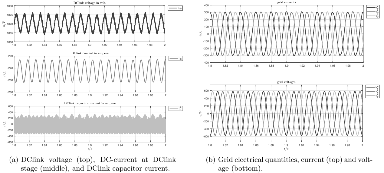
Figure 17: DC-link and grid side quantities during nominal power condition for a single ElectricalDrive connected to a i_{cc} = 50 \text{ kA} grid with MV/LV transformer with a nominal power of P_n = 1150 \text{ kVA} . As shown in the figure (a), DCLink voltage (and DC current) is affected by a sixth harmonic component (93.6 Hz) of the electrical fundamental frequency (15.6 Hz).
