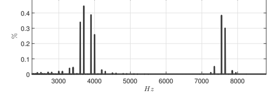
One module - grid phase current spectrum 50 \leq h \leq 160 at rated operating point - I_{ce} = 50kA
