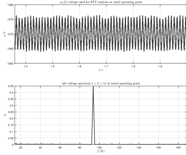
(a) DClk voltage, u_{dc}(t) , used for spectrum analysis (top); u_{dc}(t) spectrum: relevant is the 6th order component related to the 5th PSM flux component (bottom). u_{dc}^{base} = 1070 V.
