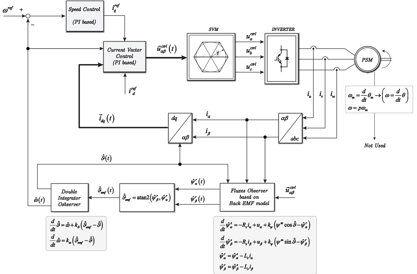
Figure 51: Control system layout of the inverter: PSM vector control with rotor phase Luemberger state observer.
