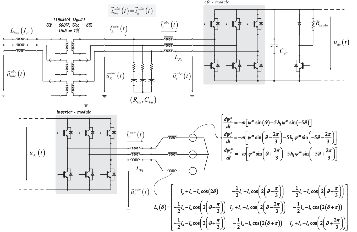
Figure 16: One ElectricalDrive case scenario used as benchmark for further investigation on modularity effect on grid power quality. As shown in the figure, a i_{cc} = 50 kA power grid has been assumed, a P_n = 1150 kVA MV/LV and an equivalent PSM three phase system with a nominal power of 250kW and a nominal current of 370A (rms). For sake of clarity, simulations have been performed supposing the grid line voltage affected by a 1% of fifth voltage harmonics as well as PSM back EMF voltage is assumed affected by a 2% of fifth voltage harmonic.
