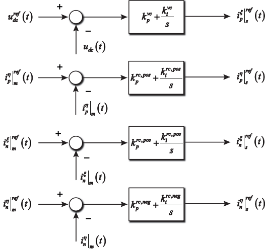
afe current components generator (outer control loops)
