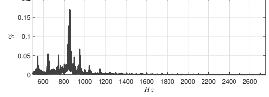
Four modules - grid phase current spectrum 50 \leq h \leq 160 at rated operating point - I_{ce} = 50kA
