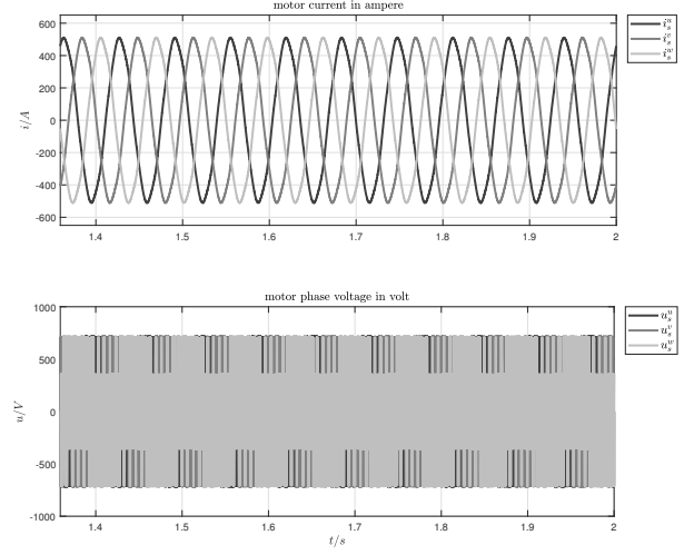
(b) inverter output current and voltage respect to the stationary reference frame, in SI.
