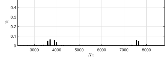
Eight modules - grid phase current spectrum 50 \leq h \leq 160 at rated operating point - I_{cc} = 50 \text{ kA}
