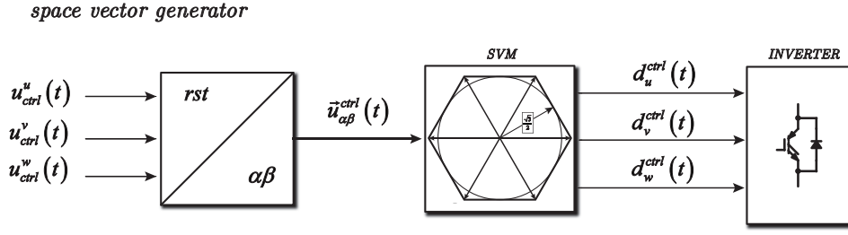
Figure 50: Space vector modulation.
