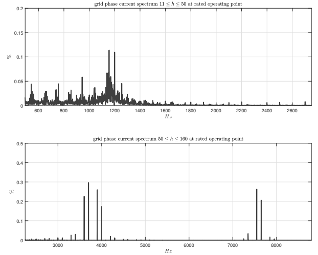
(b) grid current spectrum; effect of the resonance between equivalent grid side inductance ( L_{line} + L_{\sigma} ) and output filter capacitor of the AFE stage C_{Fu} (top); residual PWM switching harmonic current components (strongly affected by the quantity L_{line} + L_{\sigma} ) (bottom).
