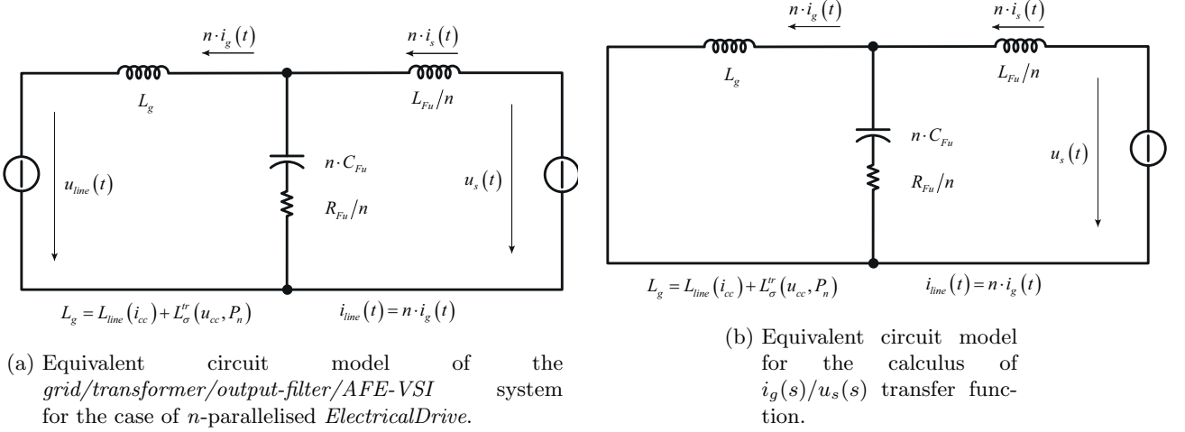
Figure 10: Equivalent circuit model (per phase equivalent star connection) of the grid/transformer/output-filter/AFE-VSI system for the case of n -parallelised ElectricalDrive (a), and equivalent circuit for the calculus of i_g(s)/u_s(s) transfer function (b).
