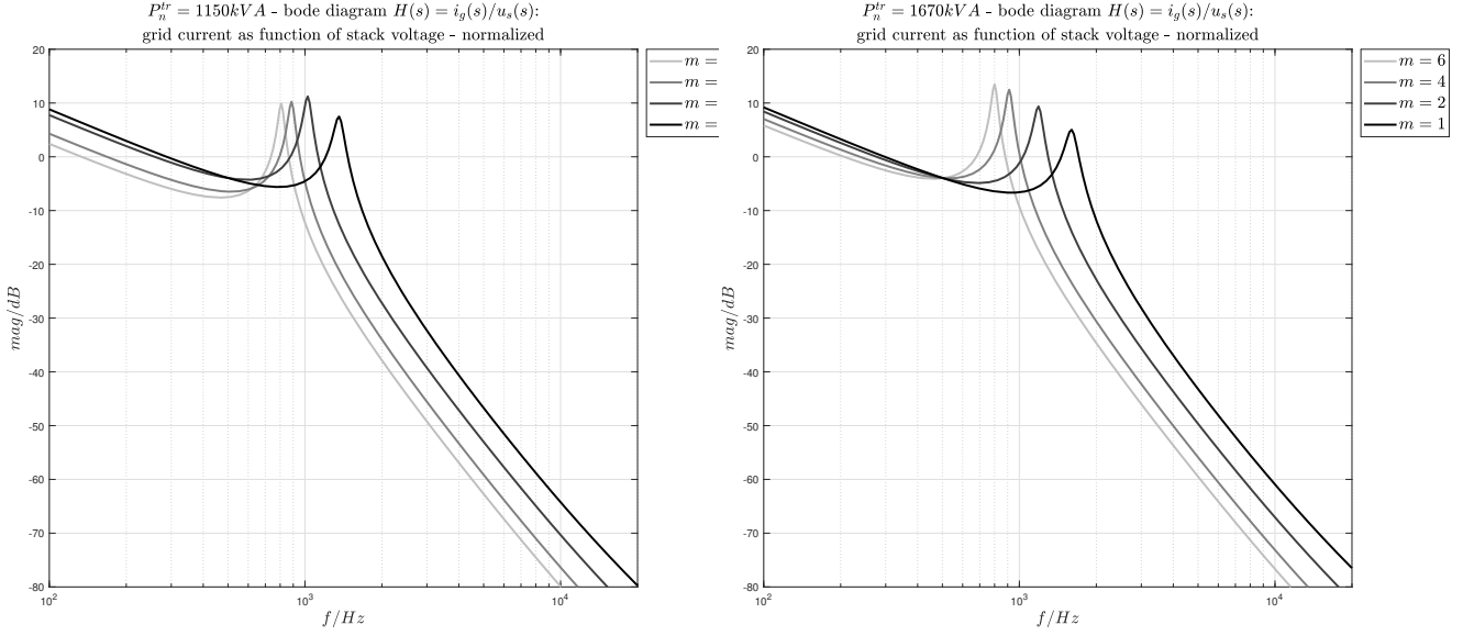
(a) Bode diagram of the equivalent of the transfer function: i_g(s)/u_s(s) , for m = 1, 2, 3, 4 modules connected to the grid via a transformer of P_n = 1150 kVA.
