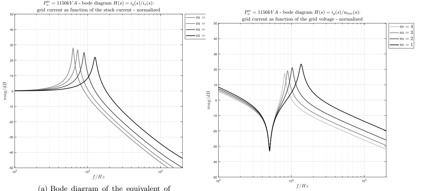
(b) Bode diagram of the equivalent of the transfer function: i_g(s)/u_{line}(s) , for m = 1, 2, 3, 4 modules connected to the grid via a transformer of P_n = 1150 \text{ kVA} .
