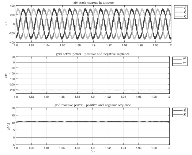
(b) afe stack current respect a stationary reference frame in SI (top); active power components in SI (middle); reactive power components in SI (bottom).
