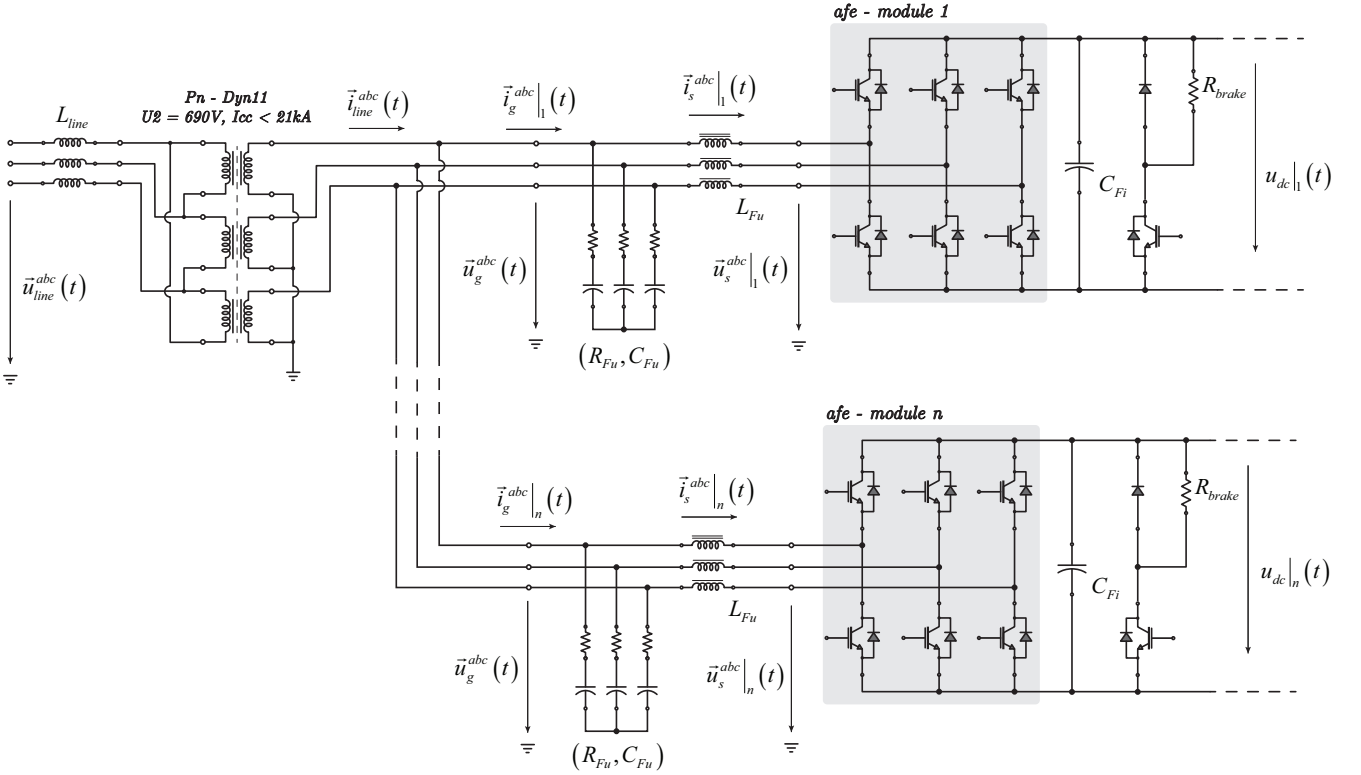
Figure 4: Electrical representation of the Grid-AFE side of the ElectricalDrive connection. Sections with subscript s , e.g. i_s^{abc}(t) concerns stack quantities while subscript g , e.g. i_g^{abc}(t) concerns grid side quantities. The pipe symbol is used to discriminate the number of the ElectricalDrive which is accounted.
