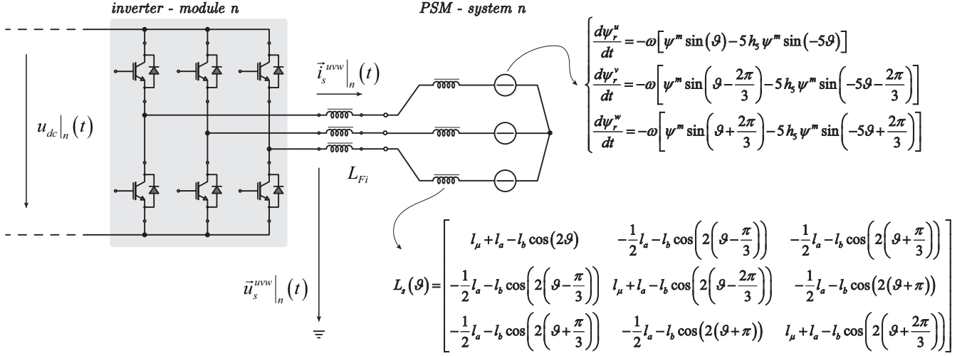
Figure 5: Electrical representation of the inverter side of the ElectricalDrive . Sections with subscript s , e.g. i_s^{uvw}(t) concerns stack quantities. The PSM representation takes into consideration the anisotropy of the magnetic circuit, equivalent matrix inductance as function of the electrical rotor position, as well as the presence the of fifth harmonic into the flux distribution. The pipe symbol is used to discriminate the number of the ElectricalDrive which is accounted.
