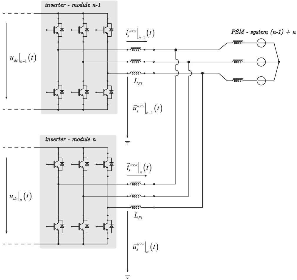
Figure 6: Electrical representation of the inverter side of the ElectricalDrive . Case scenario of hard-parallelization.
