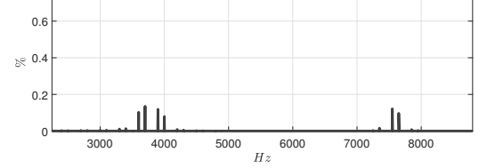
Four modules - grid phase current spectrum 50 \leq h \leq 160 at rated operating point - I_{ce} = 50kA
