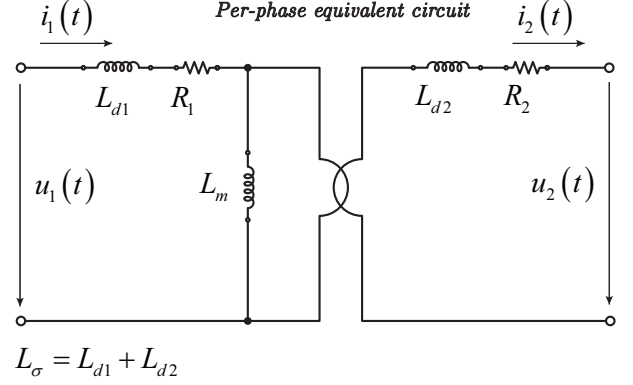
(b) Per-phase equivalent circuit of the MV/LV transformer.
