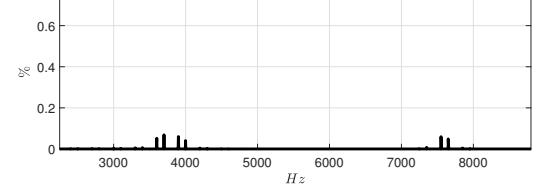
Eight modules - grid phase current spectrum 50 \leq h \leq 160 at rated operating point - I_{ce} = 50kA
