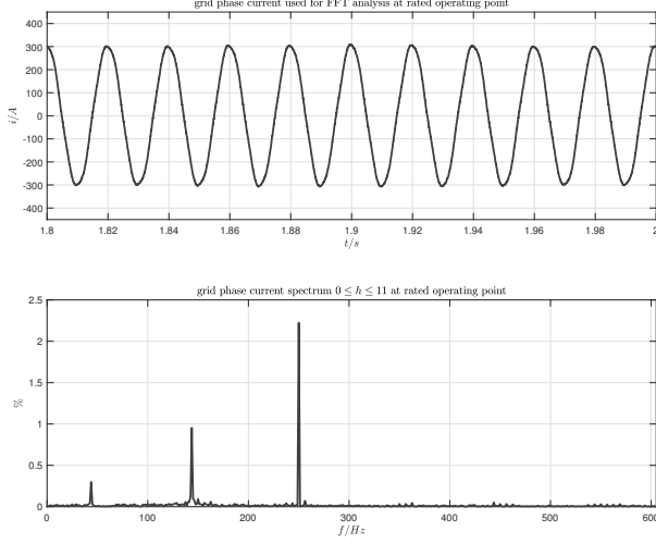
(a) grid phase current (top); grid phase current spectrum (bottom); components at 43.6 Hz and 143.6 Hz are coupled to the fifth harmonic component of the PSM back EMF; component at 250 Hz is coupled to the homologous grid voltage harmonic component.
