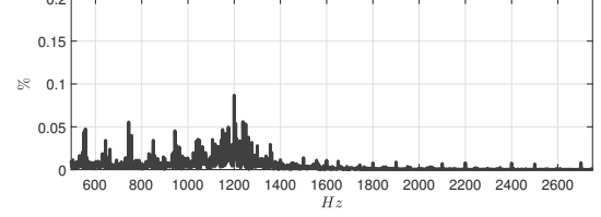
One module - grid phase current spectrum 50 \leq h \leq 160 at rated operating point - I_{ce} = 50kA
