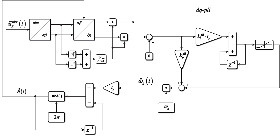
Figure 46: Control structure of the DQ-PLL. DQ-PLL is used to measure (or incorrectly saying estimated ) \hat{\omega}_g(t) and \hat{\theta}_g(t) the pulsation and the phase of the grid three phase voltage system.
