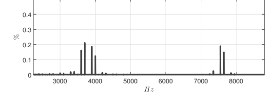
Two modules - grid phase current spectrum 50 \leq h \leq 160 at rated operating point - I_{ce} = 50kA
