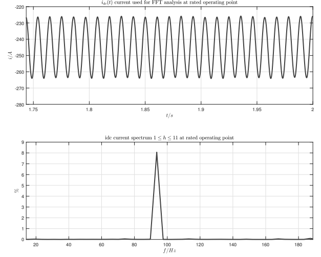
(b) DClk current, i_{dc}(t) , used for spectrum analysis (top); i_{dc}(t) spectrum: relevant is the 6th order component related to the 5th PSM flux component (bottom). i_{dc}^{base} = 234 A.
