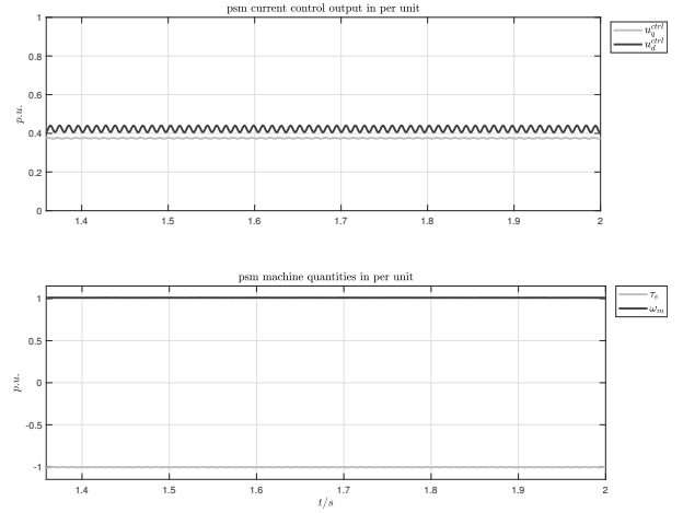
(b) per unit output current control loop: u_d^{ctrl}(k) , u_q^{ctrl}(k) respect to the rotating reference frame (top); per unit mechanical quantities: rotor speed and electromechanical torque (bottom).
