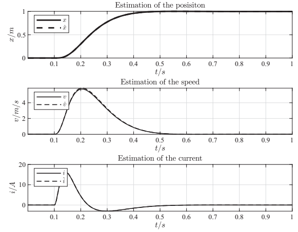
(b) Observer performance. Case (1).
