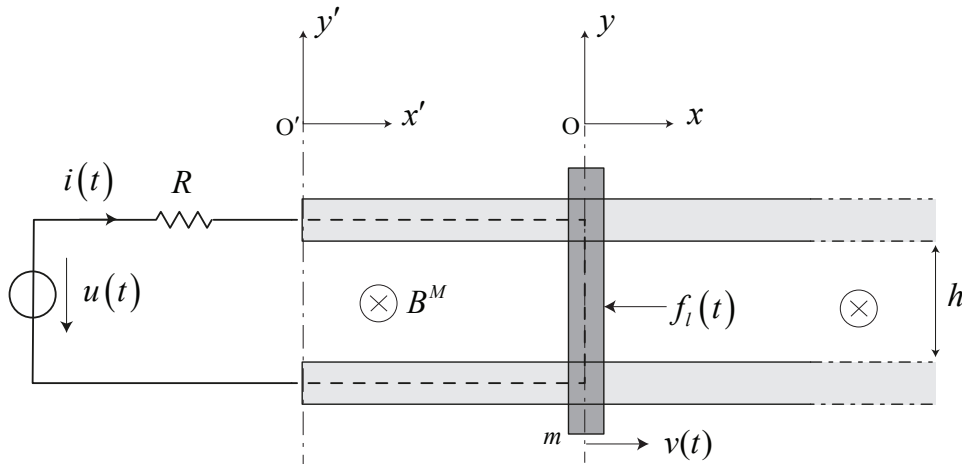
Figure 4: Linear actuator.
