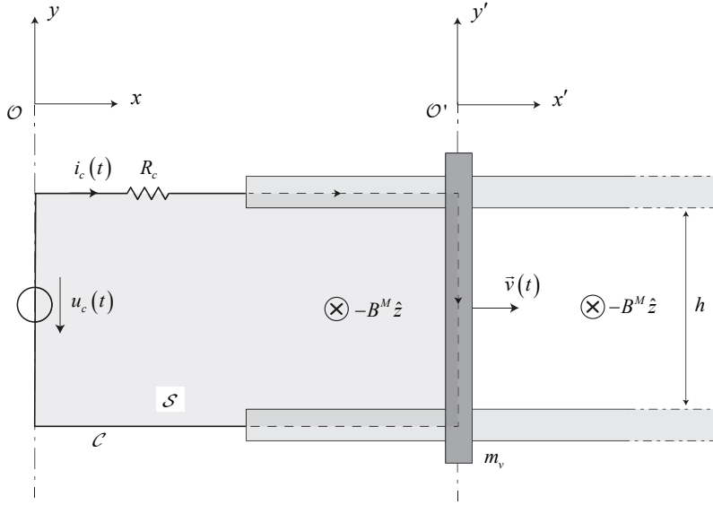
Figure 1: Moving coil actuator.
