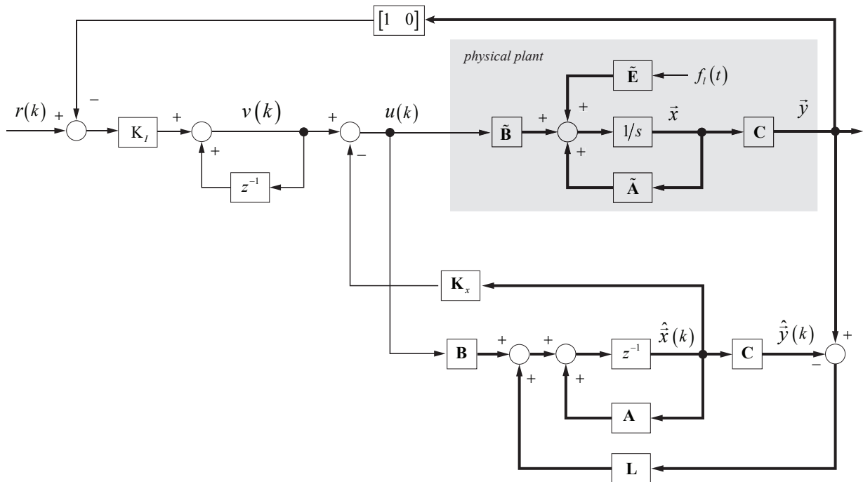
Figure 5: Control architecture.
