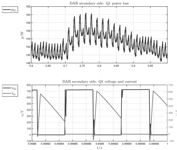
(a) Single phase DAB - secondary inverter: Q1-MOSFET power loss, voltage and current.
