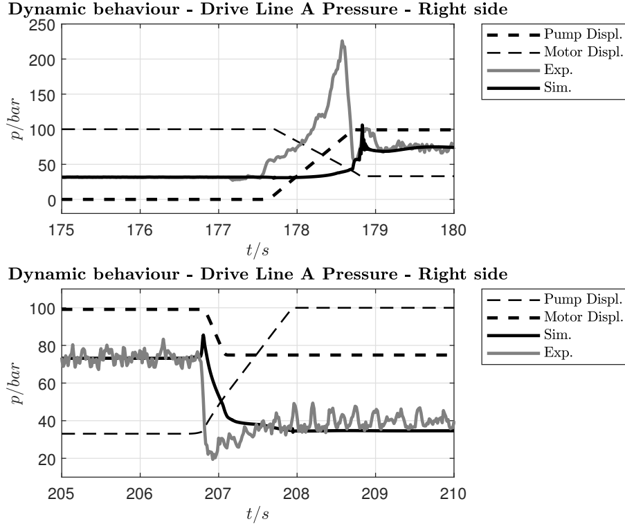
Figure 3.33: Dynamic behaviour gap between model and real vehicle in the condition of lifted case.
