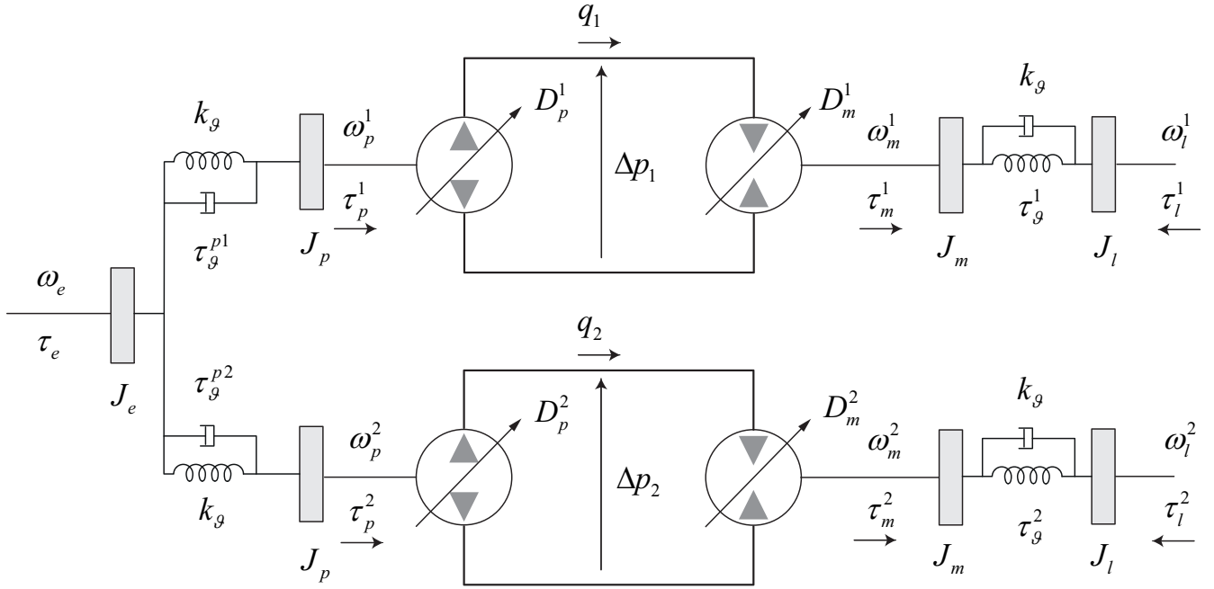
Figure 3.2: Hydrostatic transmission - no-leakage and no-viscosity case is taken into account.
