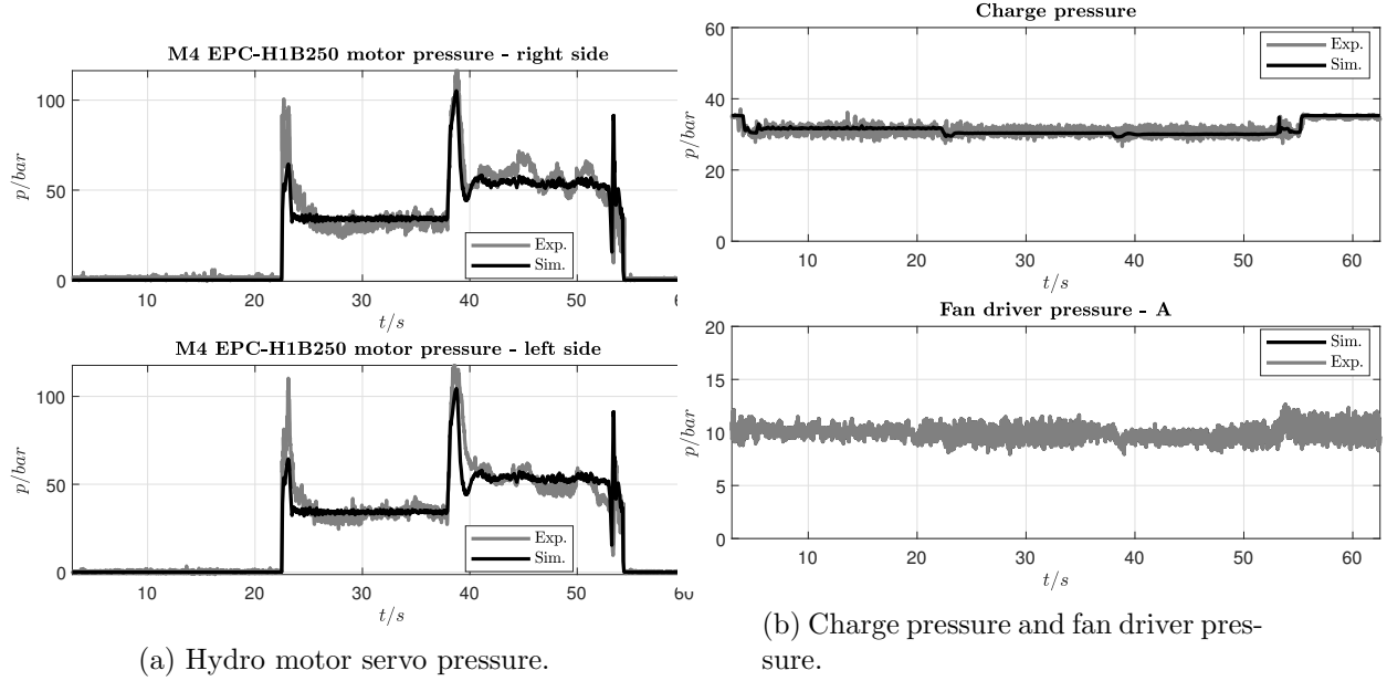
Figure 3.23: Simulation results Test 14.1.
