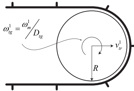
Figure 3.6: Track representation.
