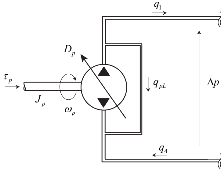
Figure 2.2: Hydrostatic pump.
