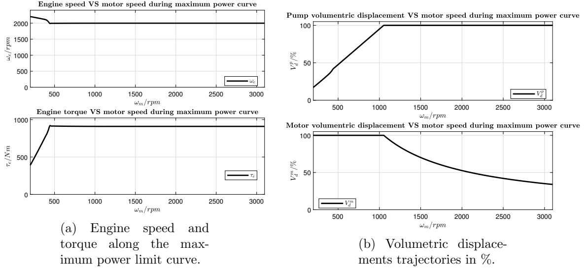
Figure 3.5: Power train limit curves - for one line.
