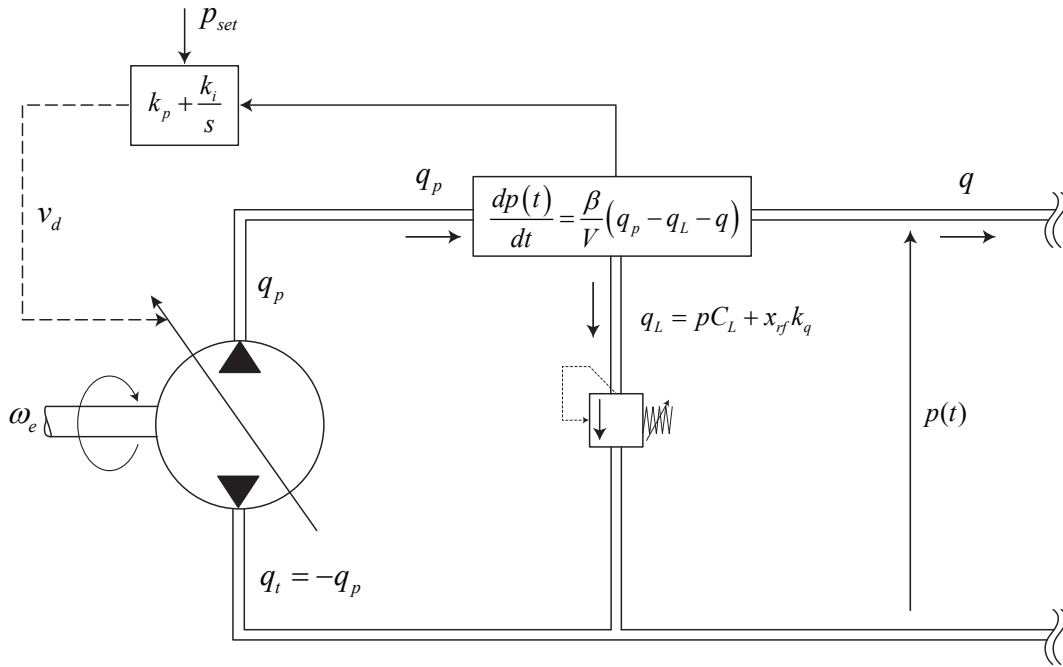
Figure 2.5: Pressure controlled pump.
