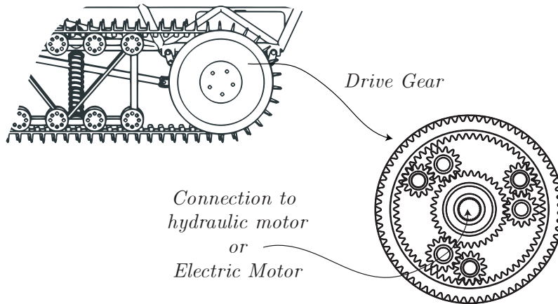
Figure 3.4: drive-gear representation.
