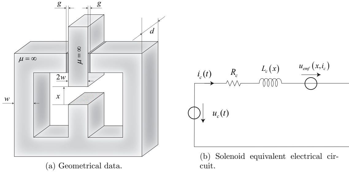
Figure 5.2: Solenoid actuator.
