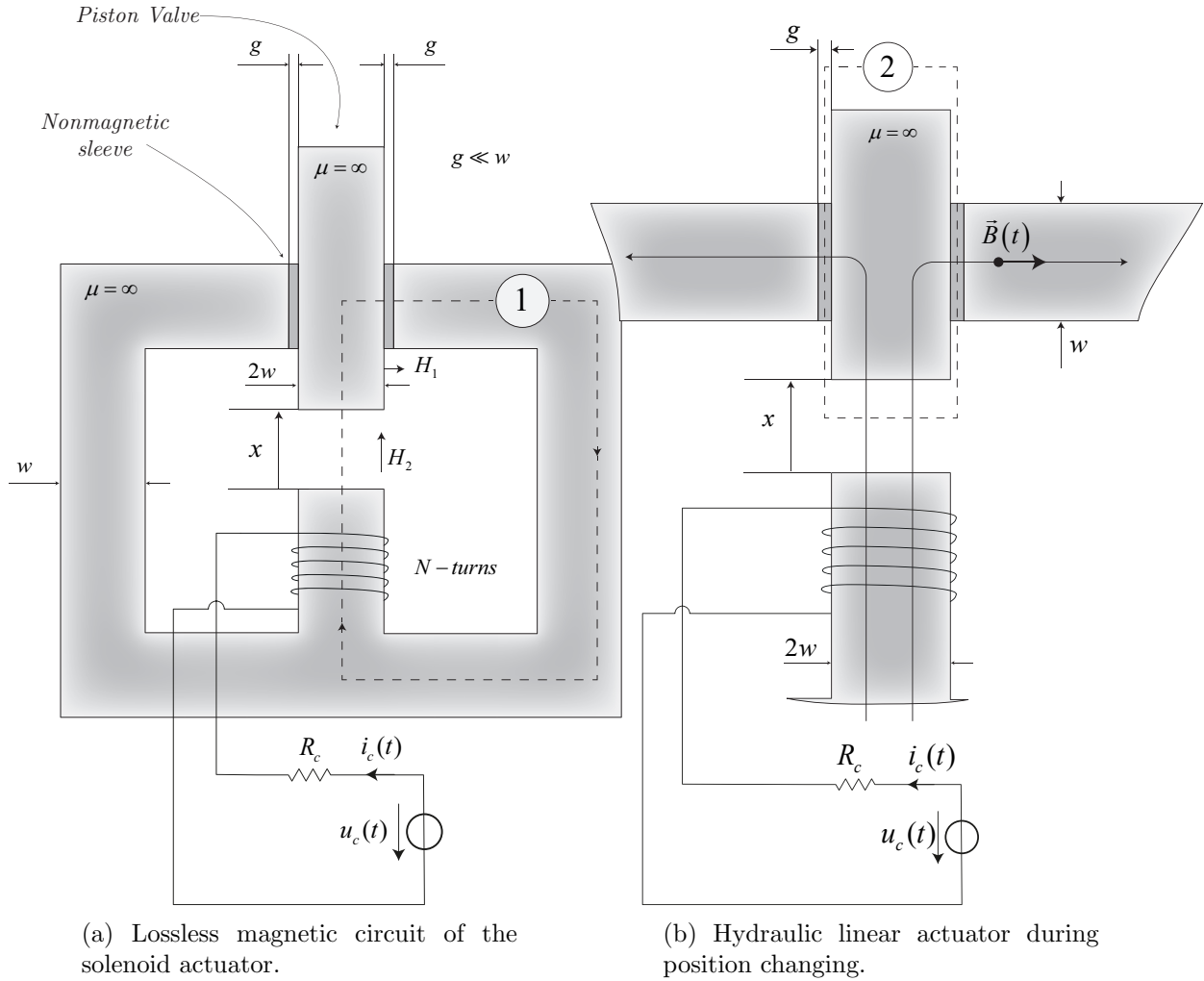
Figure 5.1: Solenoid actuator.
