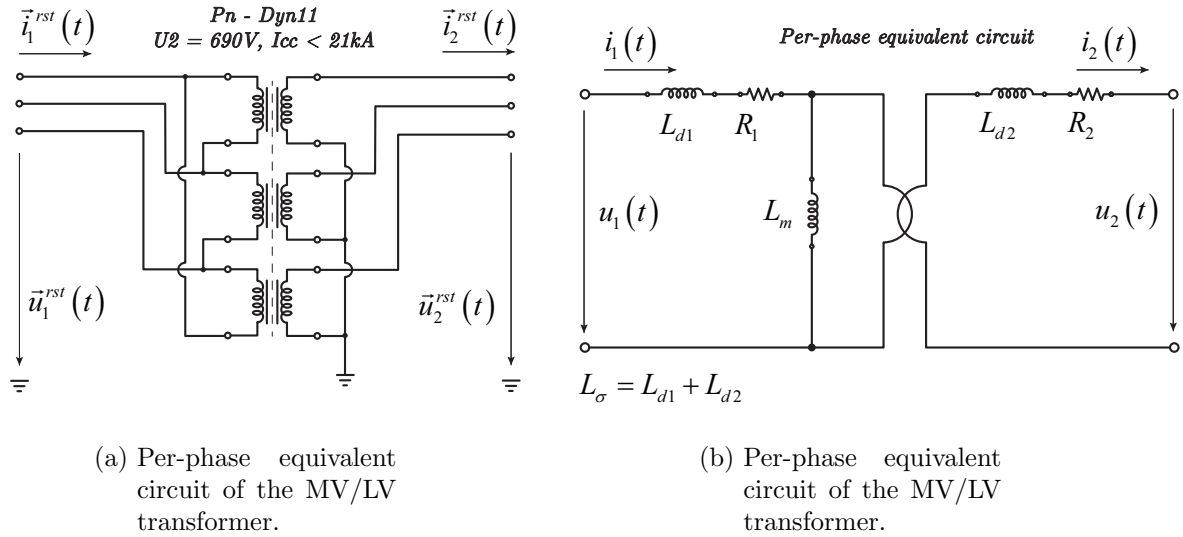
Figure 3: MV/LV main transformer; its modelization plays a fundamental role into the resulting harmonic current and power quality.
