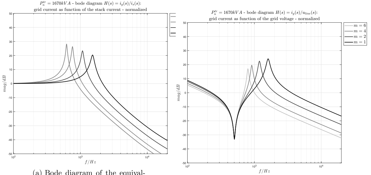
(b) Bode diagram of the equivalent of the transfer function: i_g(s)/u_{line}(s) , for m = 1, 2, 4, 6 modules connected to the grid via a transformer of P_n = 1670\text{ kVA} .
