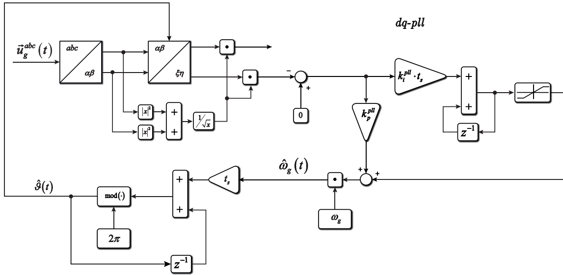
Figure 46: Control structure of the DQ-PLL. DQ-PLL is used to measure (or incorrectly saying estimated ) \hat{\omega}_g(t) and \hat{v}_g(t) the pulsation and the phase of the grid three phase voltage system.
