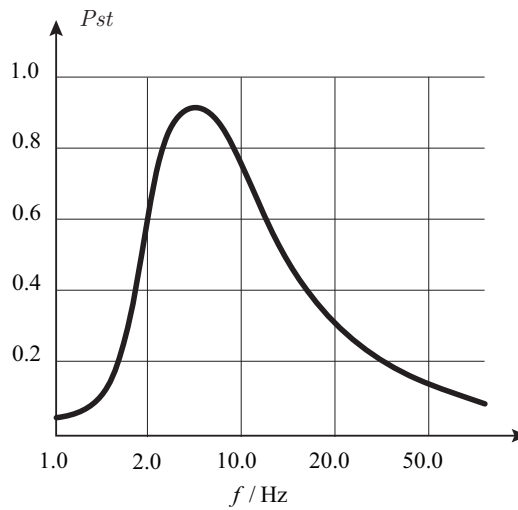
Figure 44: Flicker window severity.
