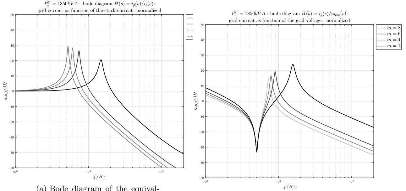
(b) Bode diagram of the equivalent of the transfer function: i_g(s)/u_{line}(s) , for m = 1, 4, 6, 8 modules connected to the grid via a transformer of P_n = 1850 kVA.
