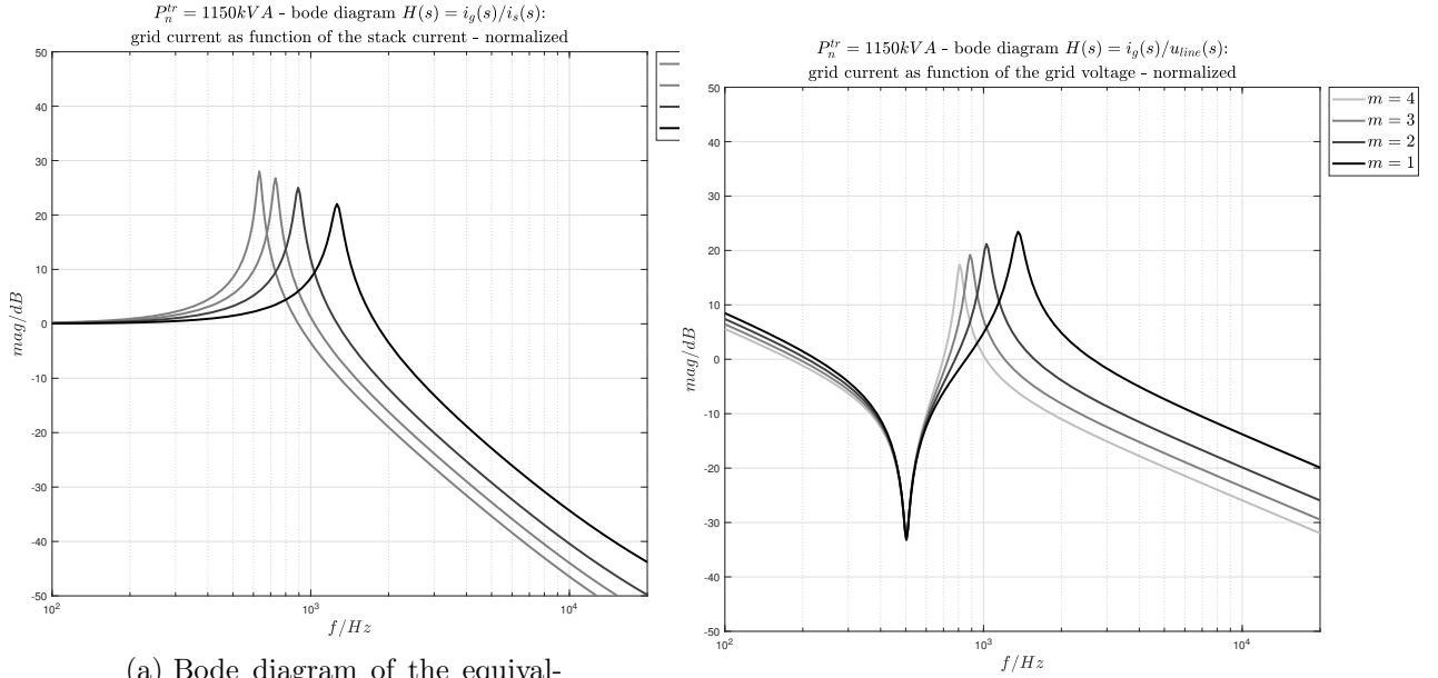
(b) Bode diagram of the equivalent of the transfer function: i_g(s)/u_{line}(s) , for m = 1, 2, 3, 4 modules connected to the grid via a transformer of P_n = 1150\text{kVA} .
