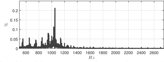
Two modules - grid phase current spectrum 50 \leq h \leq 160 at rated operating point - I_{cc} = 50kA
