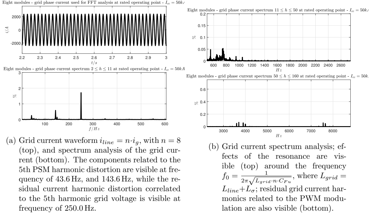
Figure 43: Case study with eight ElectricalDrive operating at 206.25kW. Current base used for normalization is i_{line}^{base}|_{m8} = \sqrt{\frac{2}{3} \frac{P_{base}}{u_{nom}}} = 1952.5 A, where P_{base} = 1650 kW, and u_{nom} = 690 V; the total residual current distortion is THD_i = 1.85 %.
