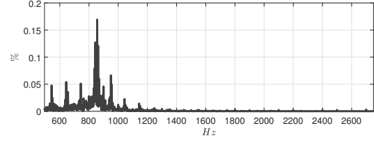
Four modules - grid phase current spectrum 50 \leq h \leq 160 at rated operating point - I_{cc} = 50kA
