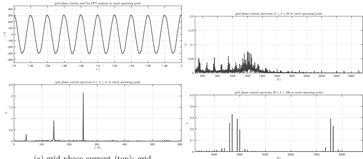
Figure 22: Grid current spectrum for the case of i_{cc} = 100 kA.
