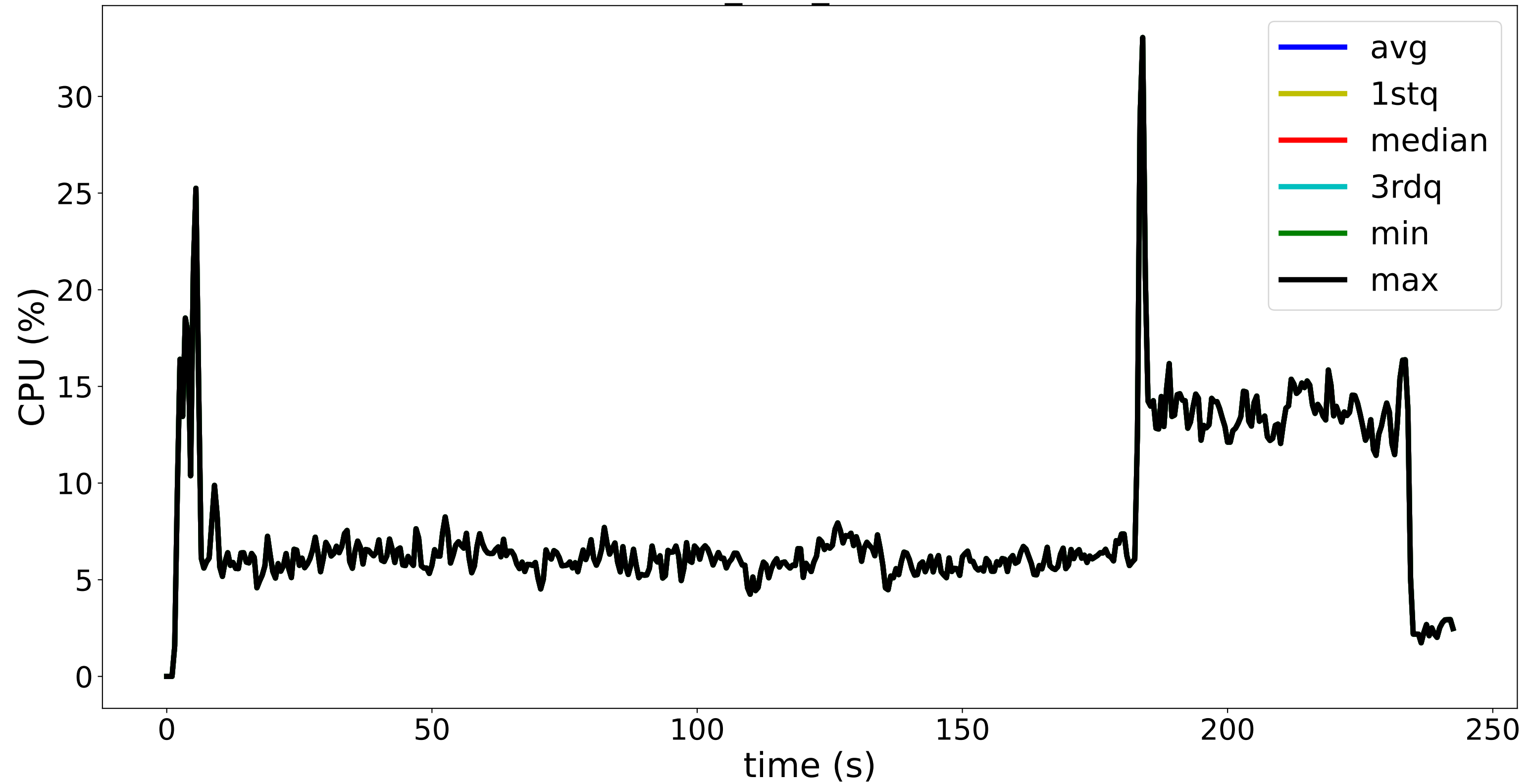
VM_CPU_USAGE
