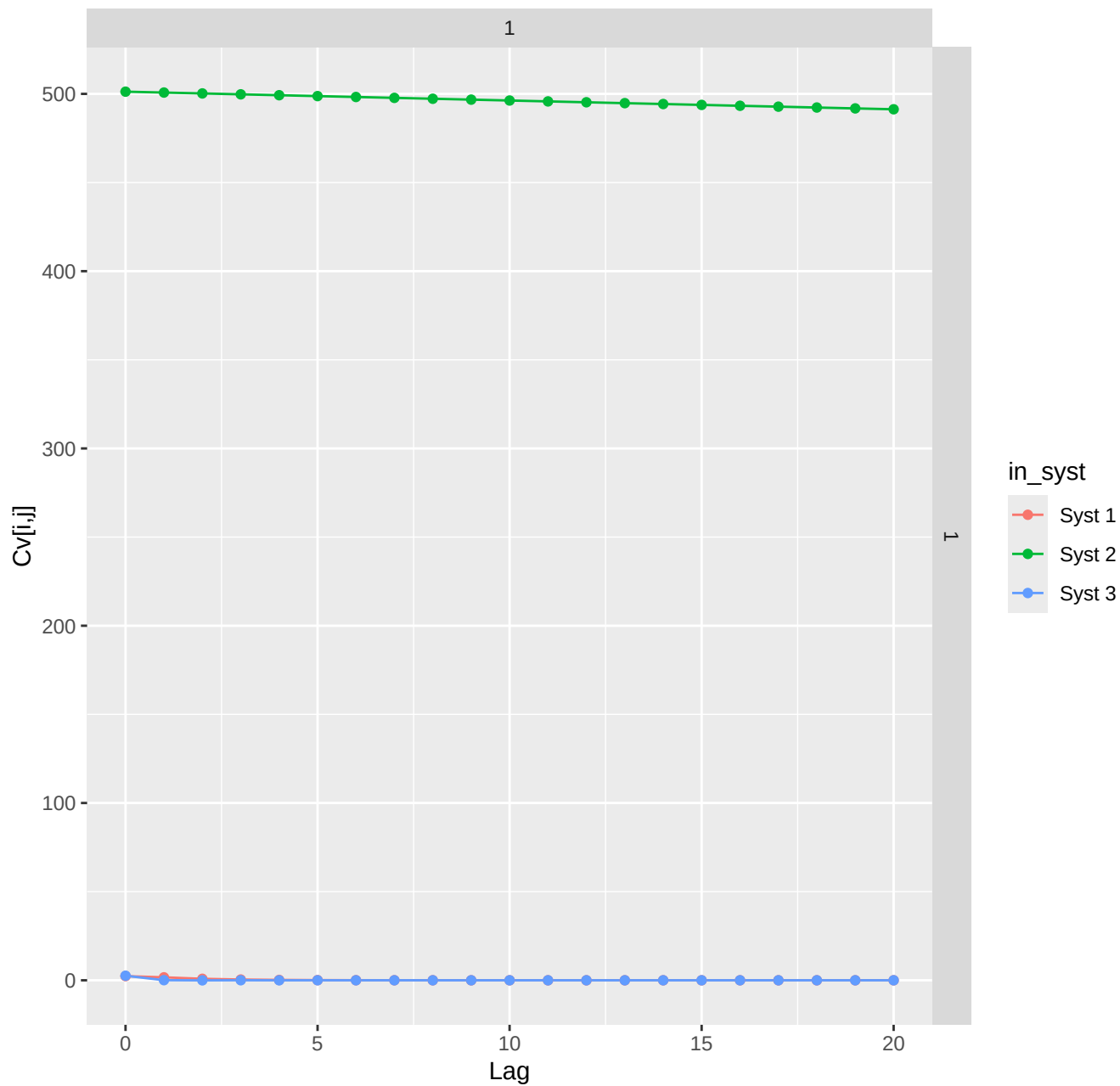
Covariance Sequence
