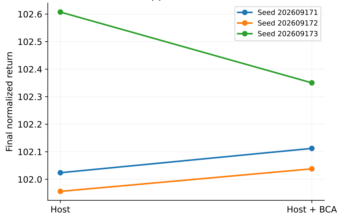
ReBRAC Hopper · 3 reviewed seeds
