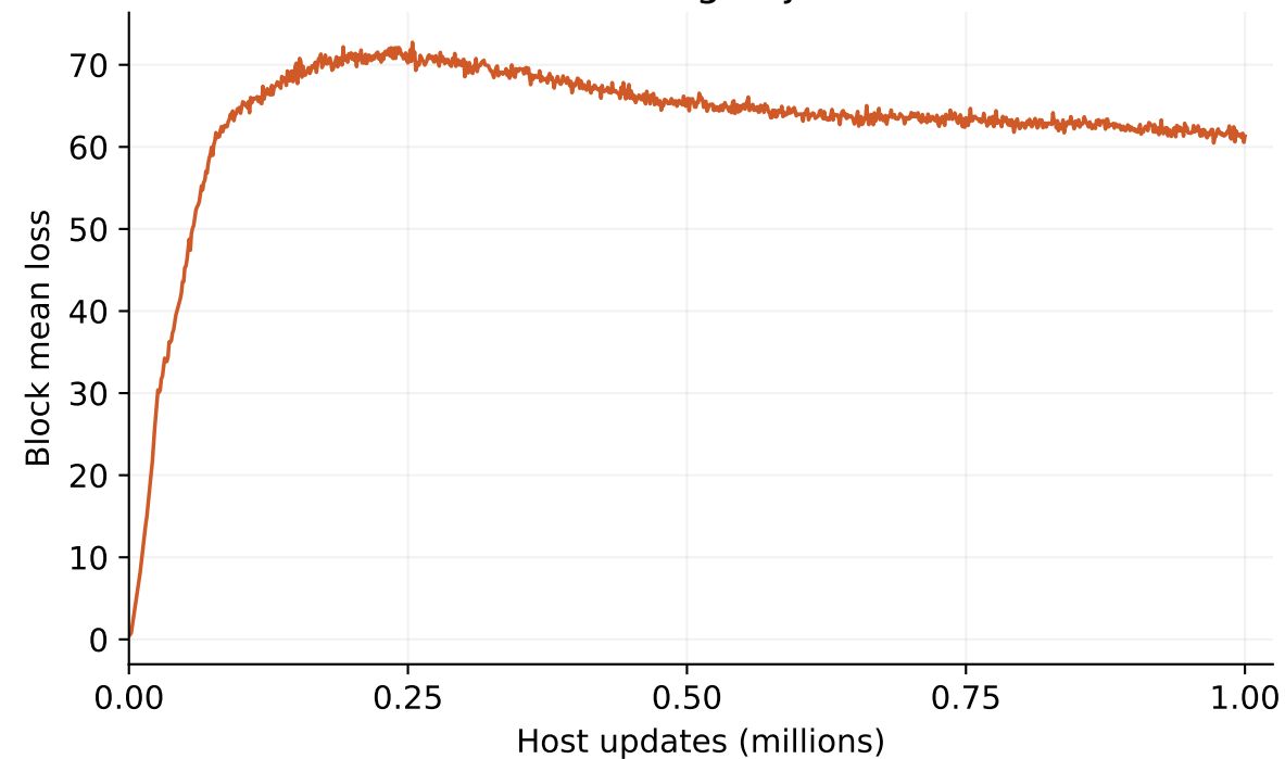
Critic fitting objective
