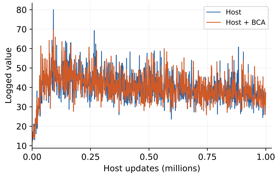
Walker · Critic 1 Bellman loss
