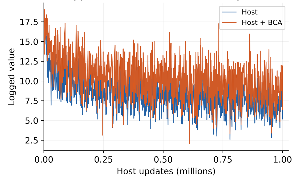
Walker · Critic 1 conservative objective
