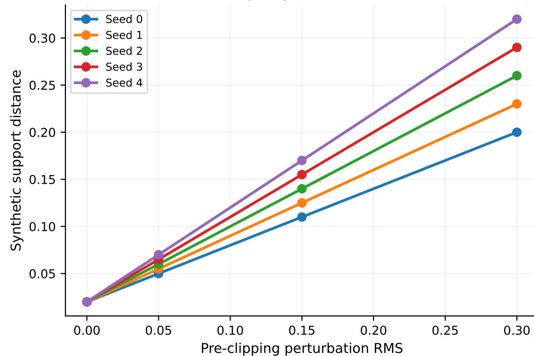
Distance is a proxy, not true OOD status
