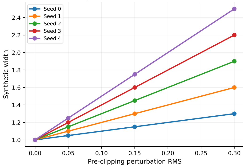
Width response to a constructed action shift
