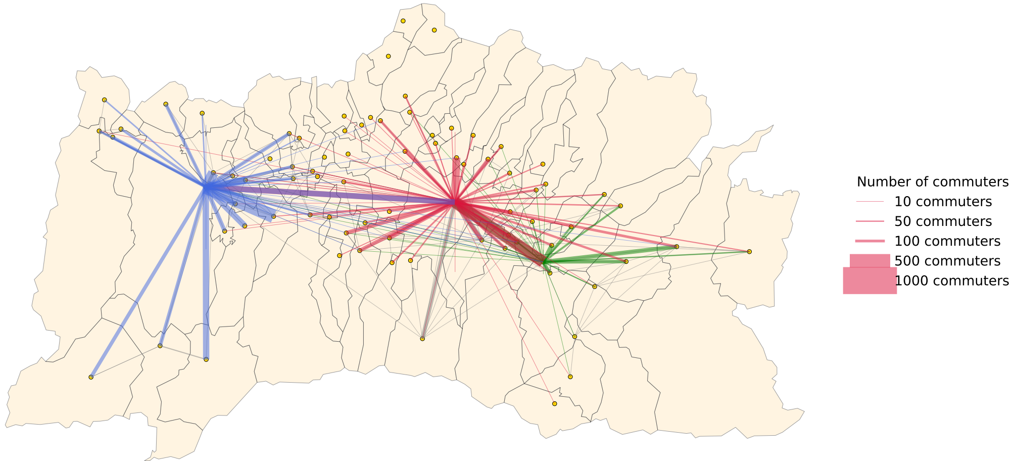
All commutes (2021)
