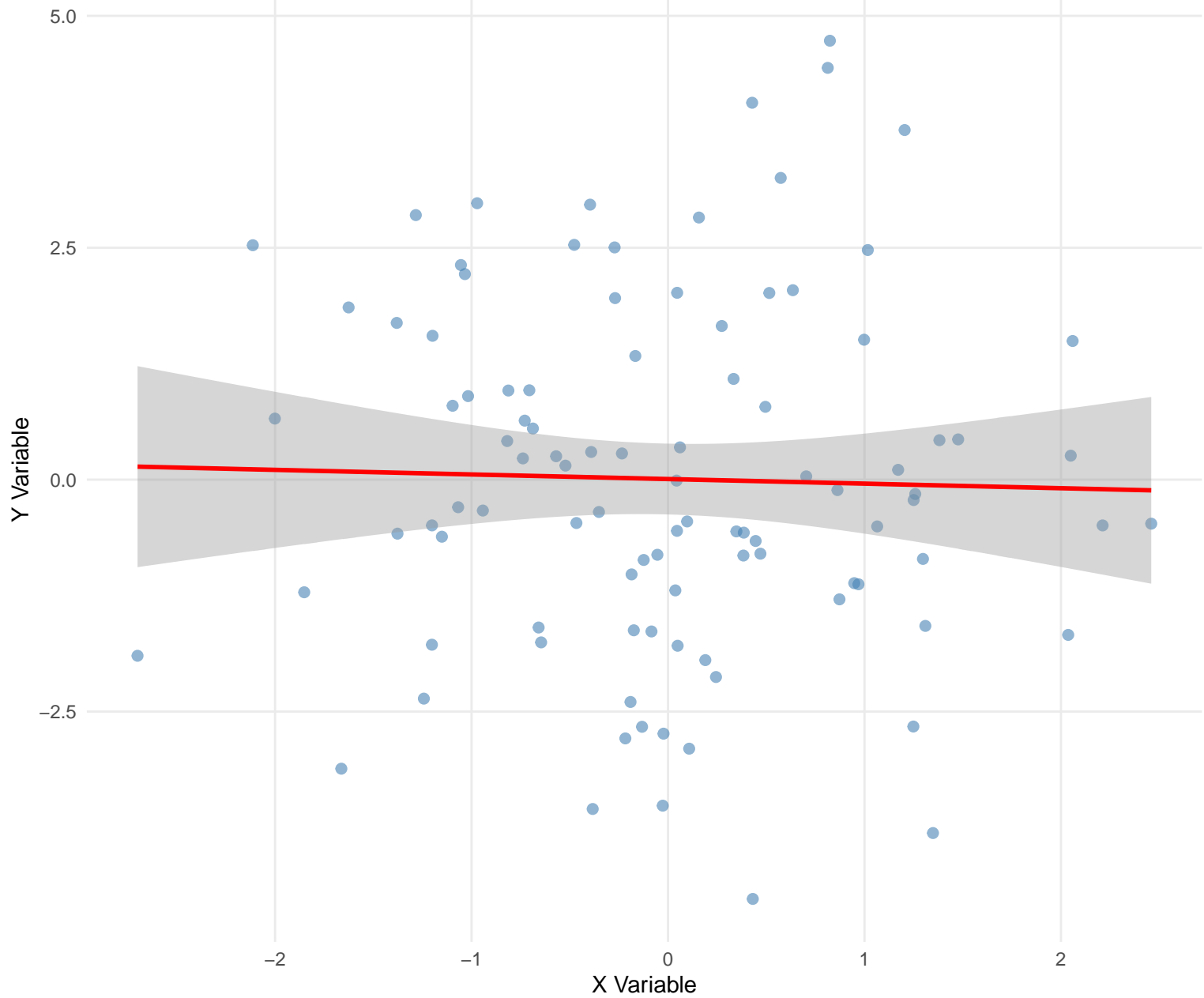
Test Scatter Plot (ggplot2)
