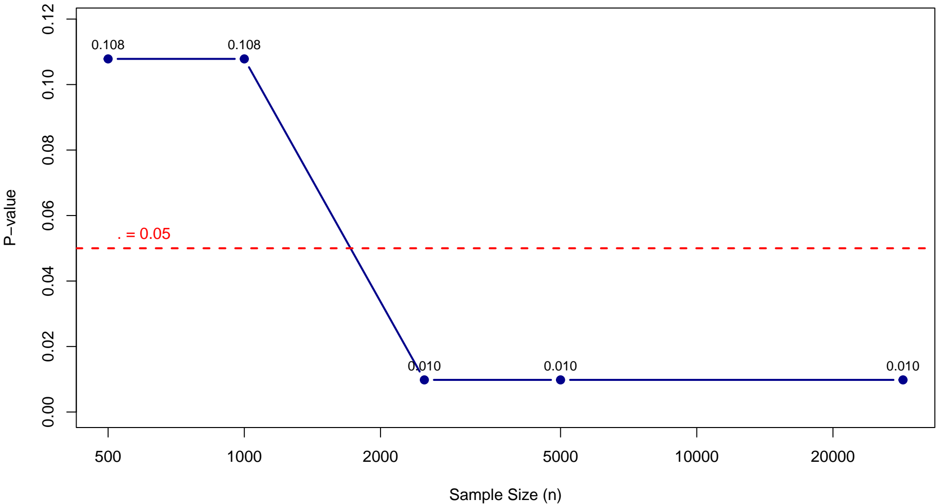
Statistical Power: P-value vs Sample Size
