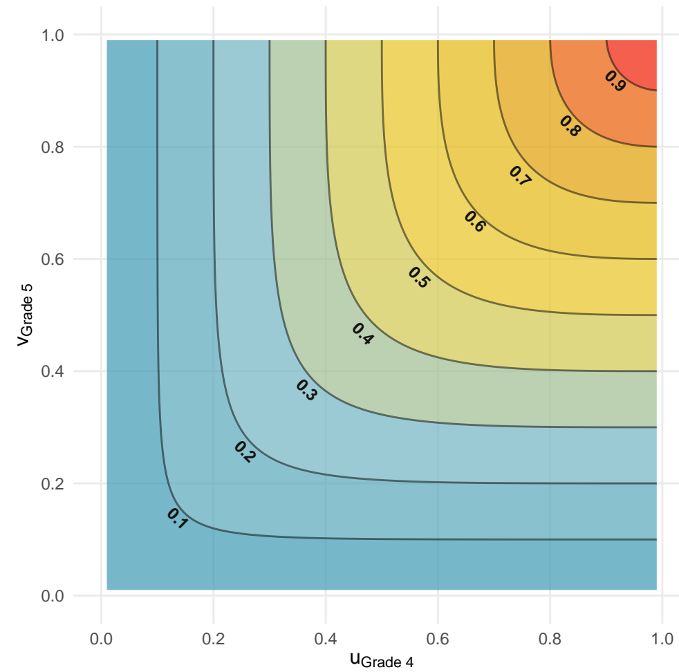
Gaussian Copula ( \tau = 0.657 , n = 51,536 )
