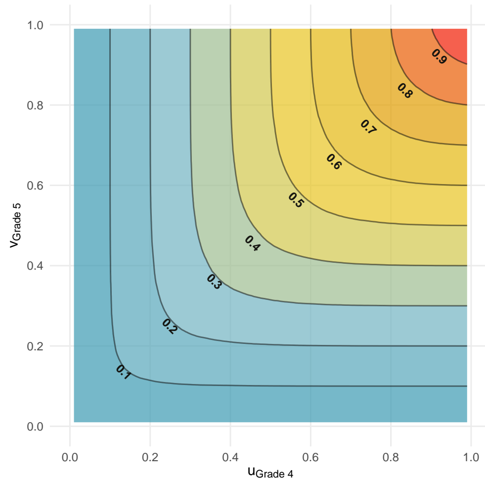
Original Score Distribution ( n = 51,536 )
