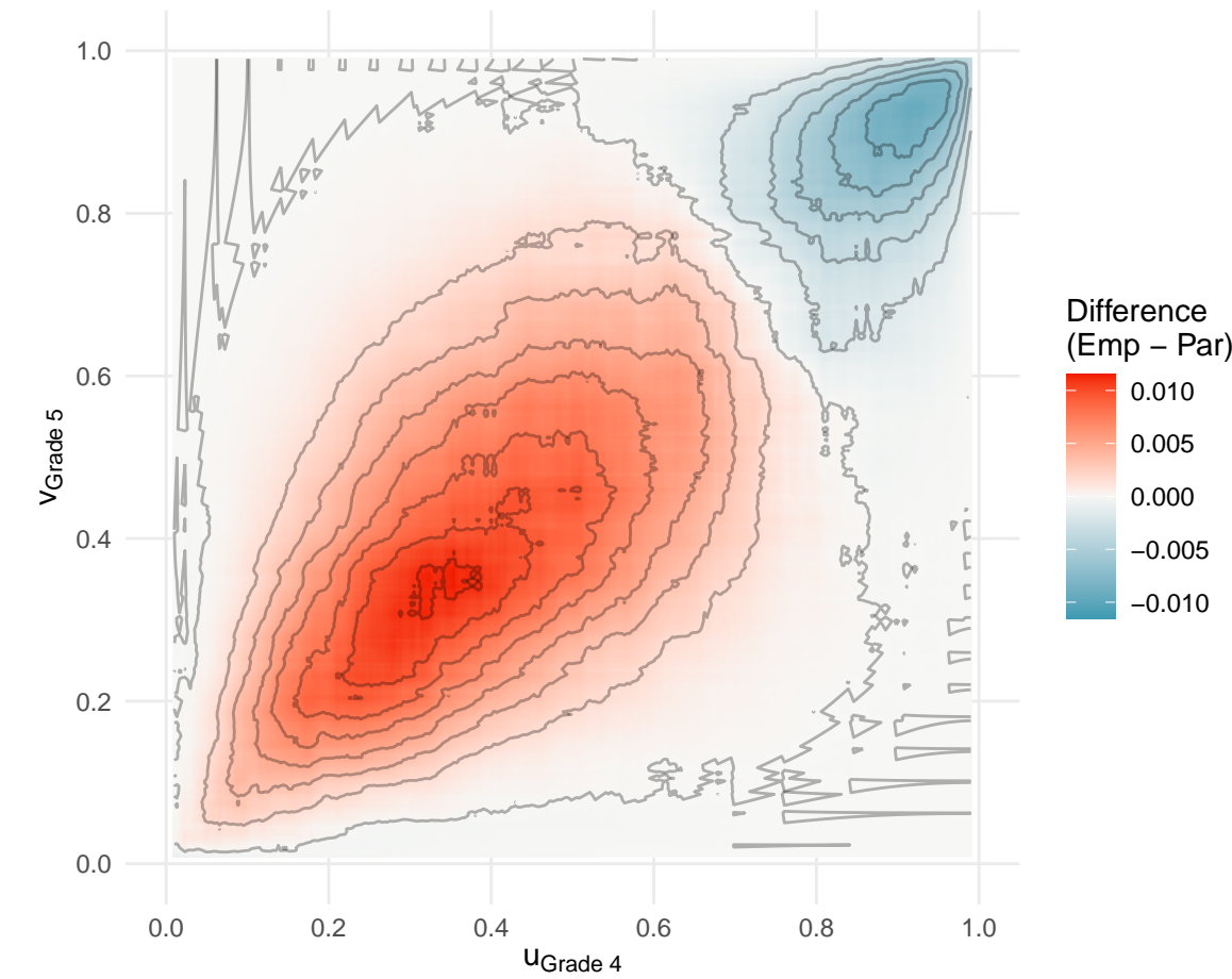
CDF Difference: Empirical – t Copula
