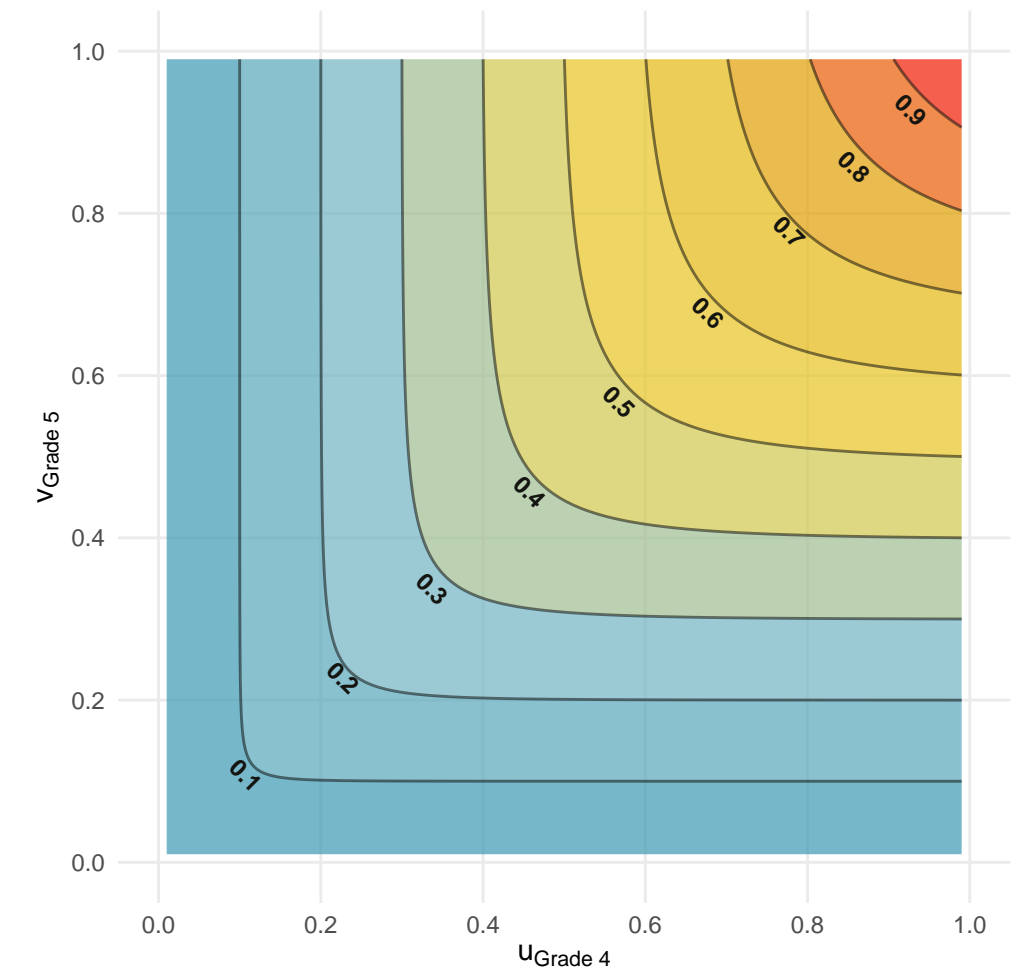
Clayton Copula ( \tau = 0.678 , n = 51,536 )
