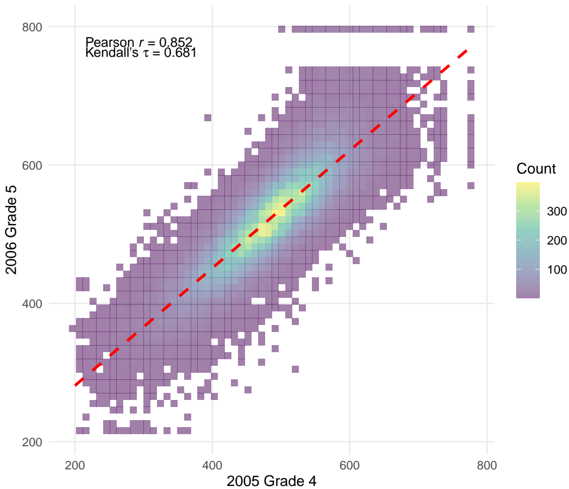
Original Score Distribution ( n = 51,536 )
