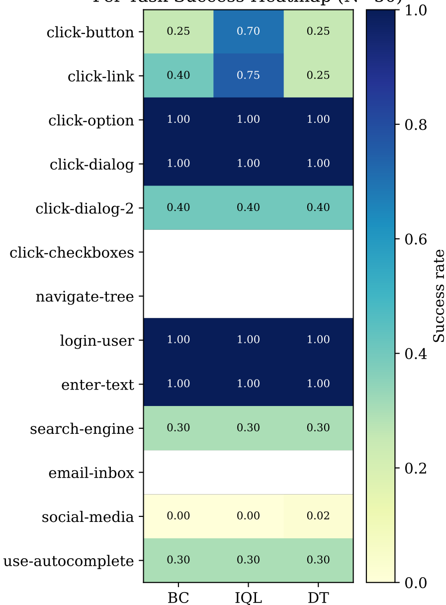
Per-Task Success Heatmap (N=50)
